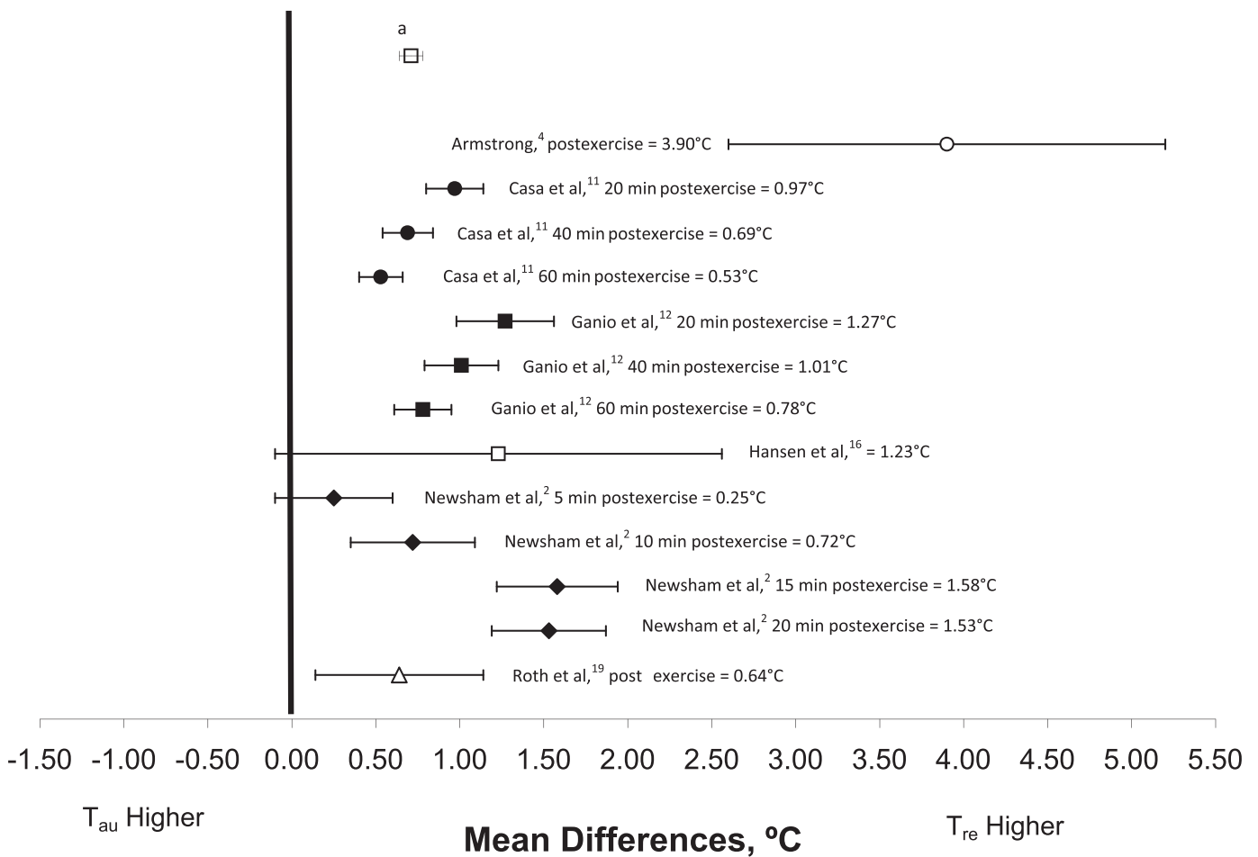
Figure 3. Mean difference (±SD) between rectal ( T_{re} ) and aural ( T_{au} ) temperatures after exercise in hyperthermic individuals. Pooled weighted mean difference reflects all included articles. a Pooled weighted mean ( T_{re} - T_{au} ) = 0.71°C.
