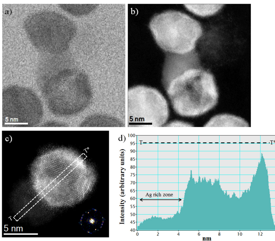
Fig. 5. (a, b) Bright field and HAADF-STEM images of AgPd/Pt hollow structure nanoparticles showing the Ag atoms are moved to the surface region and also segregated from the structure, (c) AgPd/Pt nanoparticles with an Ag rich zone (left) and Pt rich shell hollow structure (right), and (d) Intensity profile (in arbitrary units) of a typical HAADF-STEM image shows a lower magnitude on the central portion on the particle (indicated as T – T*) due to the difference in the atomic number.
