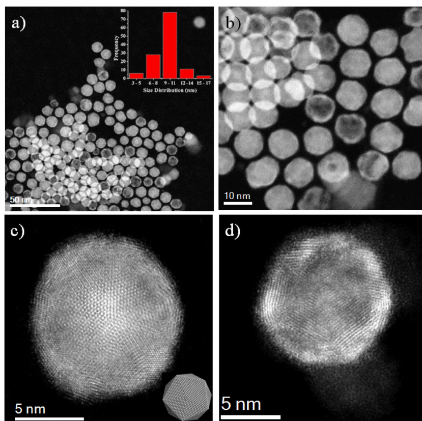
Fig. 2. (a) Low magnification and (b) Amplified HAADF-STEM images of AgPd/Pt core-shell multiply twinned particles with icosahedral morphologies. High magnification of HAADF images (c) Icosahedral structure along 5-fold symmetry axis inset shows the atomistic model of the 5-fold symmetry axis and (d) Hollow structure nanoparticle, where we observed the Ag atoms are segregated from the structure.
