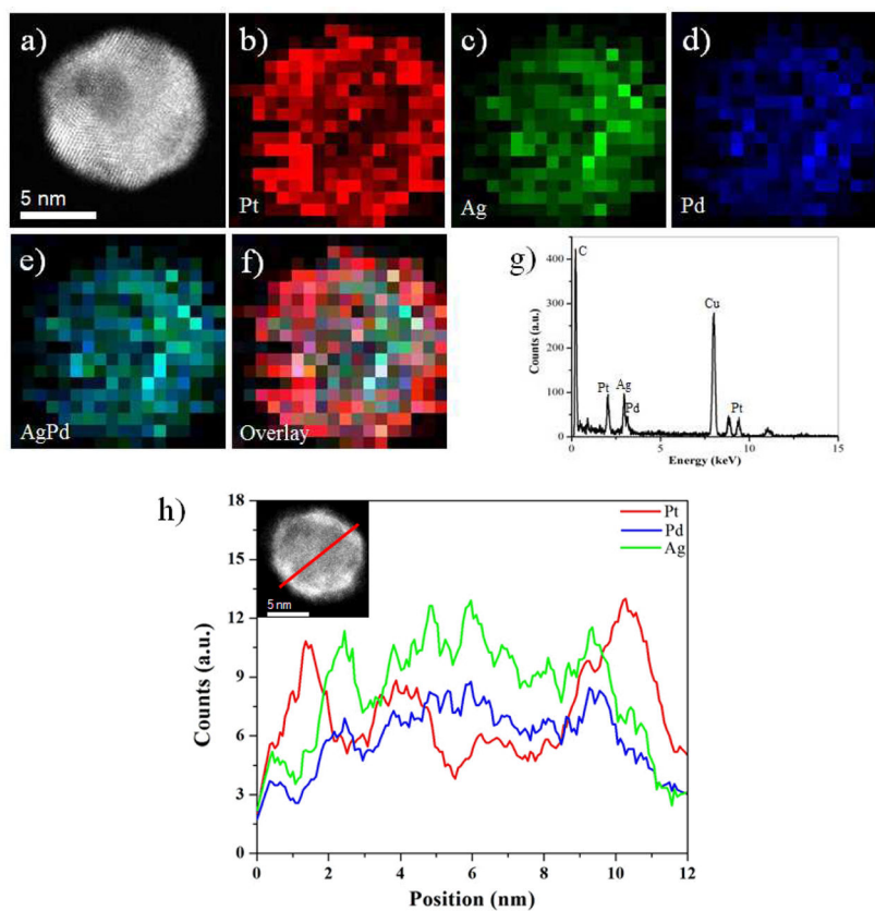
Fig. 3. (a) HAADF-STEM image of AgPd/Pt multiple twinned nanoparticles, (b–f) EDX elemental maps of nanoparticles – Pt (L, M), Ag (L), Pd (L), AgPd alloy and Overlay respectively, (g) EDX spectrum of corresponding AgPd/Pt multiply twinned nanoparticles, (h) Ag, Pd and Pt elemental profiles along the red line across the icosahedral structure (inset of h).
