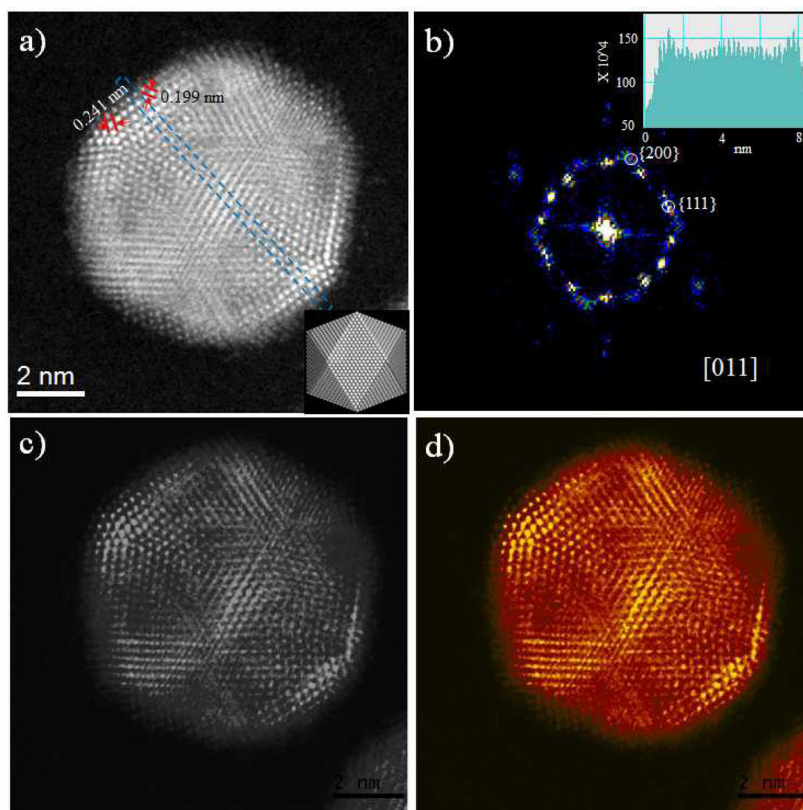
Fig. 4. Cs-corrected HAADF-STEM image of (a) AgPd/Pt nanoparticles with a Pt rich shell and AgPd rich core 2-fold symmetry axis orientated along [011] zone axis, the atomistic model is inset, (b) Fast Fourier Transform (FFT) of corresponding nanoparticles. The inset intensity profile (in arbitrary units) of the area marked in (a) showing the difference in the intensity due to the facts that Z_{Pd} < Z_{Ag} < Z_{Pt} , (c) and (d) Indicate that the different color contrast, showing the Pt shells partially covered the AgPd core surface.
