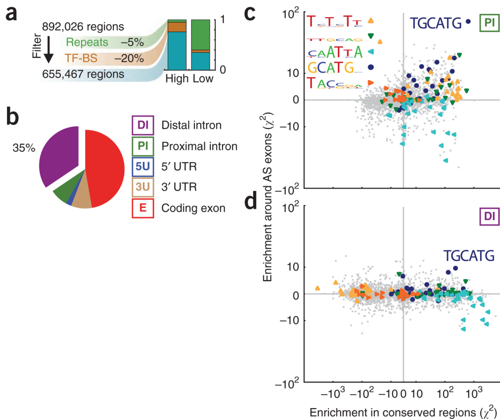
Figure 2. The Rbfox binding motif TGCATG is the most enriched hexamer in conserved regions in distal intronic space around alternatively spliced exons. (a) A flowchart of the computational strategy used to identify highly conserved regions within the human transcriptome. (b) Pie chart showing the distribution of highly conserved regions among different genes. (c,d) Scatter plot of enrichment scores for 4,096 hexamers (gray points) in proximal (c) and distal (d) intronic regions. The y axis indicates the enrichment of each word within intronic regions proximal to cassette relative to constitutive exons. The x axis indicates the enrichment of each word within highly conserved regions, relative to weakly conserved regions. The five most enriched motifs in highly conserved regions proximal to AS exons compared to weakly conserved regions proximal to constitutive exons judged by an alternative de novo approach is inset in c (additional motif information is in Supplementary Fig. 3b). Words similar to these five motifs are highlighted with filled shapes, overlaid onto the scatter plot. TGCATG was significantly ( P < 0.01 ) enriched in both proximal and distal conserved intronic regions flanking AS exons.
