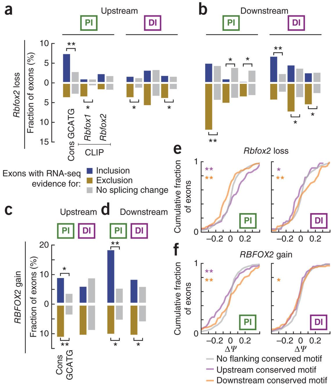
Figure 3. Both proximal and distal Rbfox motifs regulate splicing. (a–d) Bar plots depict the fraction of cassette exons for which there is evidence (listed below the first column of each panel) for direct Rbfox regulation within proximal or distal intronic regions, up or downstream (listed above each panel). Exons were classified as differentially included ( \Delta\Psi \geq 5\% ; blue, on the positive y axis), excluded ( \Delta\Psi \leq -5\% ; goldenrod reflected on the negative y axis) or not changing ( -2\% < \Delta\Psi < 2\% ; gray, on the positive and y axis and also reflected on the negative y axis) according to Rbfox2 RNA-seq experiments in mouse (a,b) and human (c,d). * P < 0.05 and ** P < 0.001 , for a Fisher’s exact test comparing the relative proportion of changed versus unaffected exons which possess a particular feature in the indicated intronic
