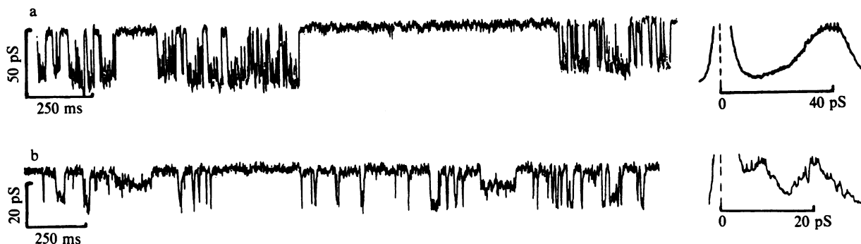
FIG. 2. Channel traces of isolated AcChoR and channel-conductance histograms ( Insets to the right) at 0.5 M Na + (buffer A) at 20°C. The bilayer was composed of soybean lipid containing 16 mol% cholesterol at a cohesive pressure of 32 mN/m. Time resolution was 1 ms. Histograms ( Insets ) were done on a 400-point probability analyzer (Honeywell, Sai-43A) with a sampling interval of 50 \mu s. Traces: a, AcChoR dimers ( \approx 50 ), recording was at 100-mV 10 min after bilayer formation and 5 min after addition of SubCho 2 (0.5 \mu M) at the cis side; b, AcChoR monomers ( \approx 50 ), recording was at 150 mV, with other conditions as in trace a.
