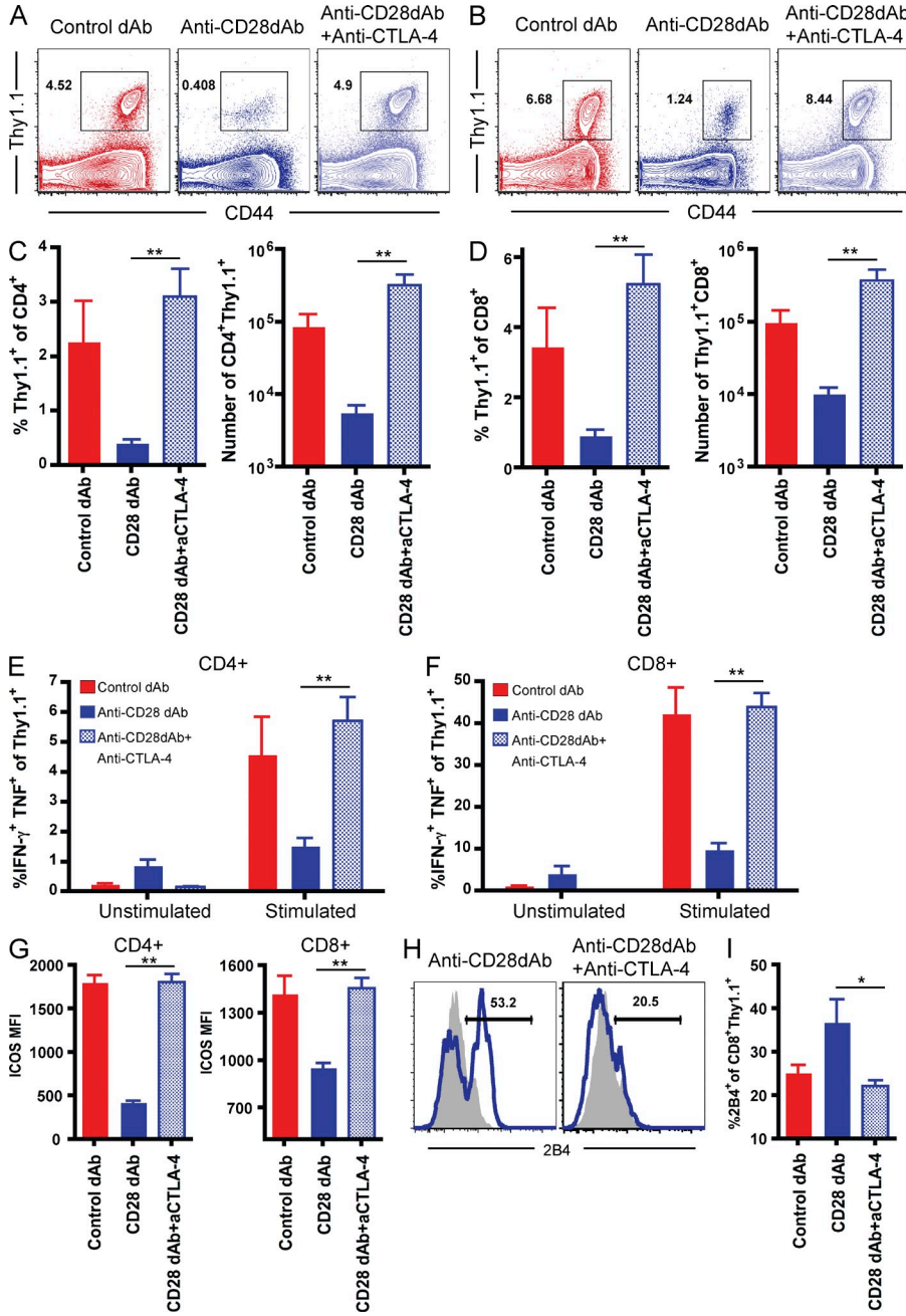
Figure 6. Increased efficacy and 2B4 up-regulation after selective CD28 blockade is dependent on CTLA-4-mediated signals. 10 6 Thy1.1 + OT-I and 10 6 Thy1.1 + OT-II T cells were adoptively transferred into naive B6 recipients, which were then challenged with an OVA-expressing skin graft in the presence of control Vκ dAb, anti-CD28 dAb, or anti-CD28 dAb + anti-CTLA-4 mAb dosed on days 0, 2, 4, and 6 as described in the Materials and methods. (A and B) Assessment of frequencies of donor-reactive CD4 + (A) and CD8 + (B) Thy1.1 + T cells on day 10 after transplant in draining lymph nodes. Data shown are representative and gated on CD4 + (A) or CD8 + (B) T cells. (C and D) Frequencies and absolute numbers of both CD4 + (C) and CD8 + (D) Thy1.1 + T cells in anti-CD28 dAb + anti-CTLA-4-treated animals as compared with animals treated with anti-CD28 dAb alone (P = 0.0079 for CD28 dAb versus CD28 dAb + anti-CTLA-4 groups). (E and F) IL-2 production by CD4 + Thy1.1 + T cells isolated from DLN on day 10 after transplant after ex vivo restimulation with OVA 323–339 (P = 0.0079 for CD28 dAb versus CD28 dAb + anti-CTLA-4 groups). (F) IFN-γ and TNF production by CD8 + Thy1.1 + T cells isolated from DLN on day 10 after transplant after ex vivo restimulation with SIINFEKL (P = 0.0079 for CD28 dAb vs. CD28 dAb + anti-CTLA-4 groups). (G) ICOS expression is shown on both CD4 + and CD8 + Thy1.1 + T cells isolated on day 10 after transplant from anti-CD28 dAb + anti-CTLA-4 treated animals relative to animals treated with anti-CD28 dAb alone (P = 0.0079). (H and I) 2B4 expression is shown on CD8 + Thy1.1 + T cells isolated on day 10 after transplant from anti-CD28 dAb + anti-CTLA-4-treated animals relative to animals treated with anti-CD28 dAb alone (P = 0.0159). All graphs are summary data of 2 independent experiments with a total of 8–10 mice per group. *, P < 0.05; **, P < 0.01.
