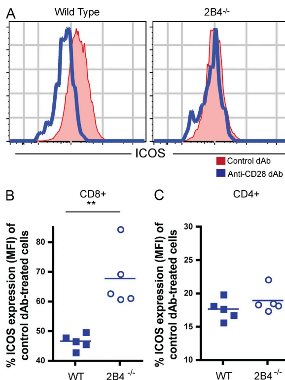
Figure 9. Reduced up-regulation of ICOS after selective CD28 blockade is dependent on engagement of the 2B4 pathway. 10 6 Thy1.1 + OT-I or 10 6 Thy1.1 + 2B4 -/- OT-I and 10 6 Thy1.1 + OT-II T cells were adoptively transferred into naive B6 recipients, which were then challenged with an OVA-expressing skin graft in the presence of control dAb or anti-CD28 dAb, and then dosed on days 0, 2, 4, and 6 and three times per week continuously thereafter as described in the Materials and methods. Graft-draining LNs were harvested on day 10 after transplant and analyzed by flow cytometry. (A) ICOS expression on WT (left) and 2B4 -/- (right) donor-reactive CD8 + Thy1.1 + T cells in the presence and absence of anti-CD28 dAb. (B) Summary data from n = 5/group (representative of 2 independent experiments with a total of 10 mice per group) show the percent reduction in ICOS expression after anti-CD28 dAb treatment as compared with control dAb treatment in WT versus 2B4 -/- CD8 + T cells ( P = 0.0018). Data shown are gated on CD8 + Thy1.1 + T cells. (C) Percent reduction in ICOS expression after anti-CD28 dAb treatment on CD4 + donor-reactive T cells in mice that received WT or 2B4 -/- OT-I T cells. Data shown are gated on CD4 + Thy1.1 + T cells. Summary data shown are from n = 5/group (representative of two independent experiments with a total of 10 mice per group). **, P < 0.01.
