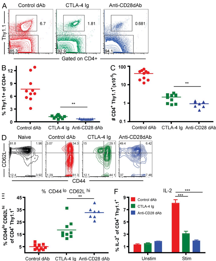
Figure 2. Donor-reactive \text{CD4}^+ T cell accumulation and differentiation are more profoundly attenuated by selective CD28 blockade versus CTLA-4 Ig. 10^6 Thy1.1 + OT-I and 10^6 Thy1.1 + OT-II T cells were adoptively transferred into naive B6 recipients, which were then challenged with an OVA-expressing skin graft in the presence of control \text{V}\kappa dAb, CTLA-4 Ig, or anti-CD28 dAb, and then dosed on days 0, 2, 4, and 6 and three times per week continuously thereafter, as described in the Materials and methods. (A) Assessment of frequencies of donor-reactive \text{CD4}^+ Thy1.1 + T cells on day 10 after transplant in draining lymph nodes. Data shown are representative and gated on \text{CD4}^+ T cells. (B and C) Summary data of 3 independent experiments with a total of 8–10 mice per group. Frequencies (B) and absolute numbers (C) of \text{CD4}^+ Thy1.1 + T cells in anti-CD28 dAb-treated animals as compared with CTLA-4 Ig-treated animals (B, P = 0.0031 ; C, P = 0.00185 ). (D) Analysis of CD44 and CD62L expression on \text{CD4}^+ Thy1.1 + T cells in DLN on day 10 after transplant. Data shown are representative. (E) Summary data of 3 independent experiments with a total of 8–10 mice per group ( P = 0.0004 ). (F) IL-2 production by \text{CD4}^+ Thy1.1 + T cells isolated from DLN on day 10 after transplant after ex vivo restimulation with OVA 323–339 ( P < 0.0001 ). **, P < 0.01 ; ***, P < 0.001 .
