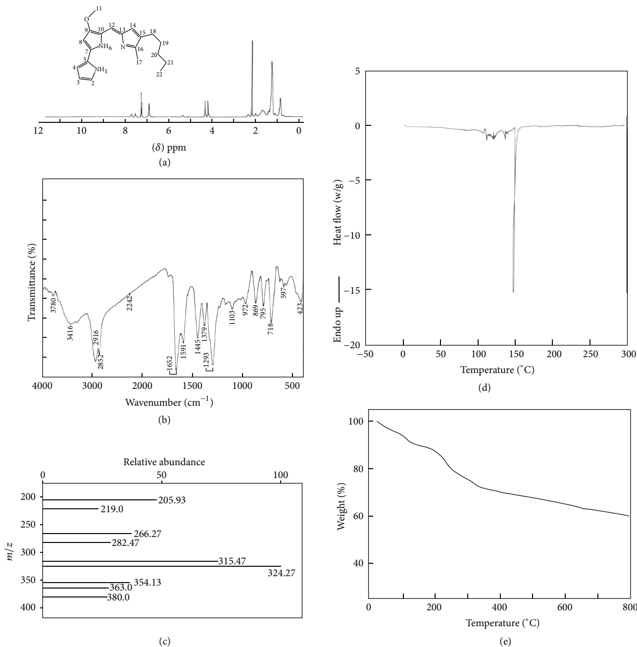
FIGURE 3: (a) Nuclear magnetic resonance spectrum of purified prodigiosin. (b) Fourier transform infra red spectrum of purified prodigiosin. (c) Electropray Ionisation-mass spectrometry analysis of purified prodigiosin. (d) Differential scanning calorimetric analysis of purified prodigiosin. (e) Thermo gravimetric analysis of purified prodigiosin.
