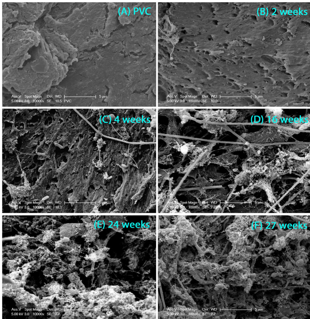
Fig. 1. SEM images of (A) PVC, (B) 2-week old biofilm, (C) 4-week old biofilm, (D) 16-week old biofilm, (E) 24-week old biofilm, and (F) 27-week old biofilm at magnification of 10,000 \times . All biofilm samples were fixed, dried, and coated with Au before imaging.
