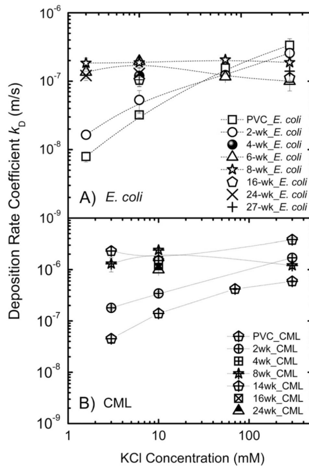
Fig. 5. Adhesion rate coefficient ( k_d ) of A) E. coli S17, and B) CML on clean PVC and biofilm surface grown at different times as a function of ionic strength (KCl) at pH 8.2–8.5 and at 25 °C. The error bars correspond to 95% confidence intervals.
