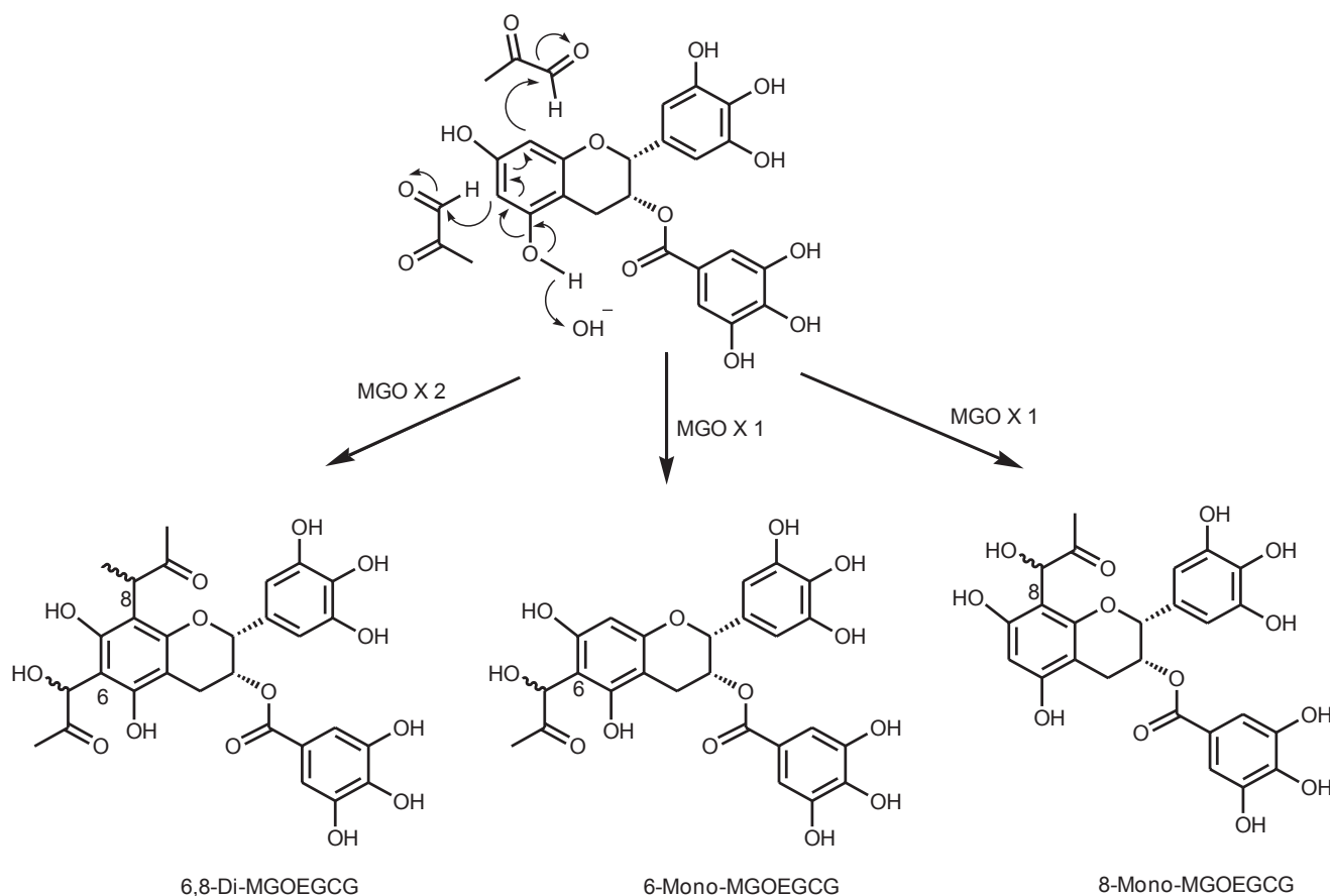
Figure 1. Adducts of methylglyoxal and epigallocatechin-3-gallate
