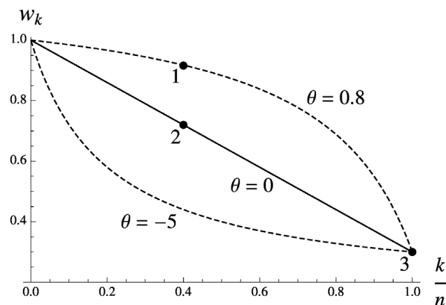
Figure 2. Genotype fitness as a function of the block length. The fitness of the genotype w_k is plotted against the proportion of the chromosome \frac{k}{n} occupied by the foreign genes: \theta=0 corresponds to additive fitness (no epistasis), while \theta=-5 and \theta=0.8 represent the positive and the negative epistasis, correspondingly. The points indicate the fitness of the initial block carrying 4 genes ( k_{\pi}=4 ) at \theta=0.8 . Point 1: n=10 , fitness is calculated according to eq. 12. Point 2: n=10 , fitness is rescaled by the length of the initial block. Point 3: initial block carries the maximum number of genes, k_{\pi}=n=4 . doi:10.1371/journal.pone.0088651.g002
