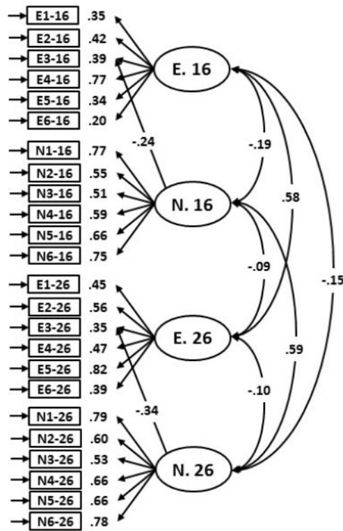
Figure 1. Personality measurement model diagram.
