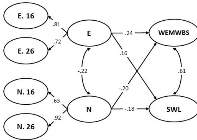
Figure 3. Structural diagram for the main effects between personality and wellbeing. E.16 = Extraversion measured at age 16; E.26 = Extraversion measured at age 26; N.16= Neuroticism measured at age 16; N.26=Neuroticism measured at age 26. E= Extraversion; N=Neuroticism; WEMWBS= Warwick-Edinburgh Mental Wellbeing Scale total score; SWL=Satisfaction with Life total score... Parameter estimates are standardized and significant at a minimum p < .05 .
