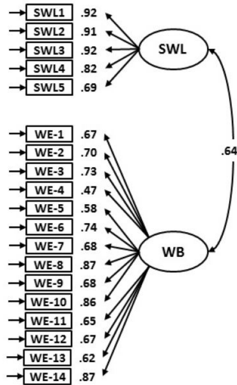
Figure 2. Well-being measurement model diagram.
