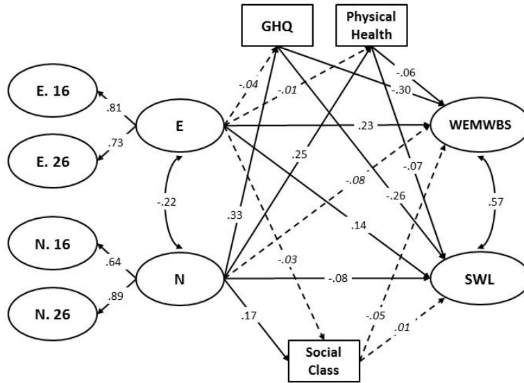
Figure 4. Full structural diagram of the latent variable associations.
