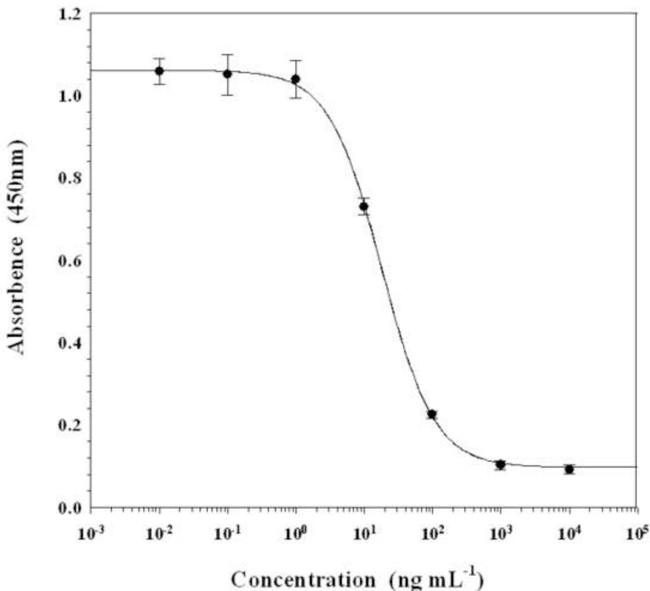
Fig. 3. ELISA standard curve for chlorpyrifos by indirect competitive assay. Assay conditions: monoclonal antibody (4B) against Hapten B-KLH, diluted 1/2700; coating antigen, Hapten A-OVA, 25 ng/well; goat anti-mouse IgG-HRP, 1/3000; organic cosolvent, 20% methanol; phosphate buffer, 100 mM; pH 7.4. Each point represents the mean of 16 determinations. Vertical bars indicate \pm standard deviation about the mean.
