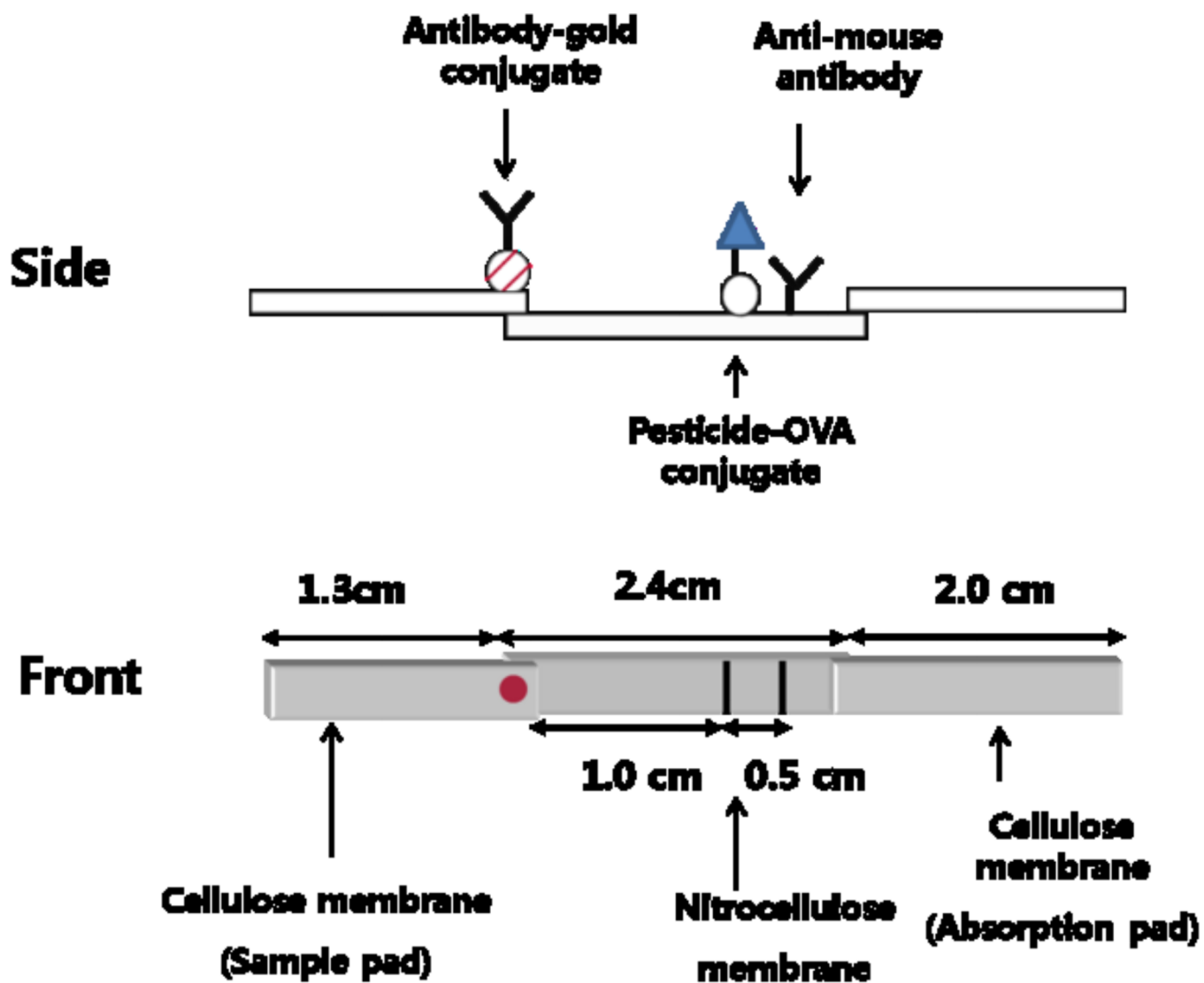
Fig. 1. Schematic diagram of the lateral flow ICA test strip.
