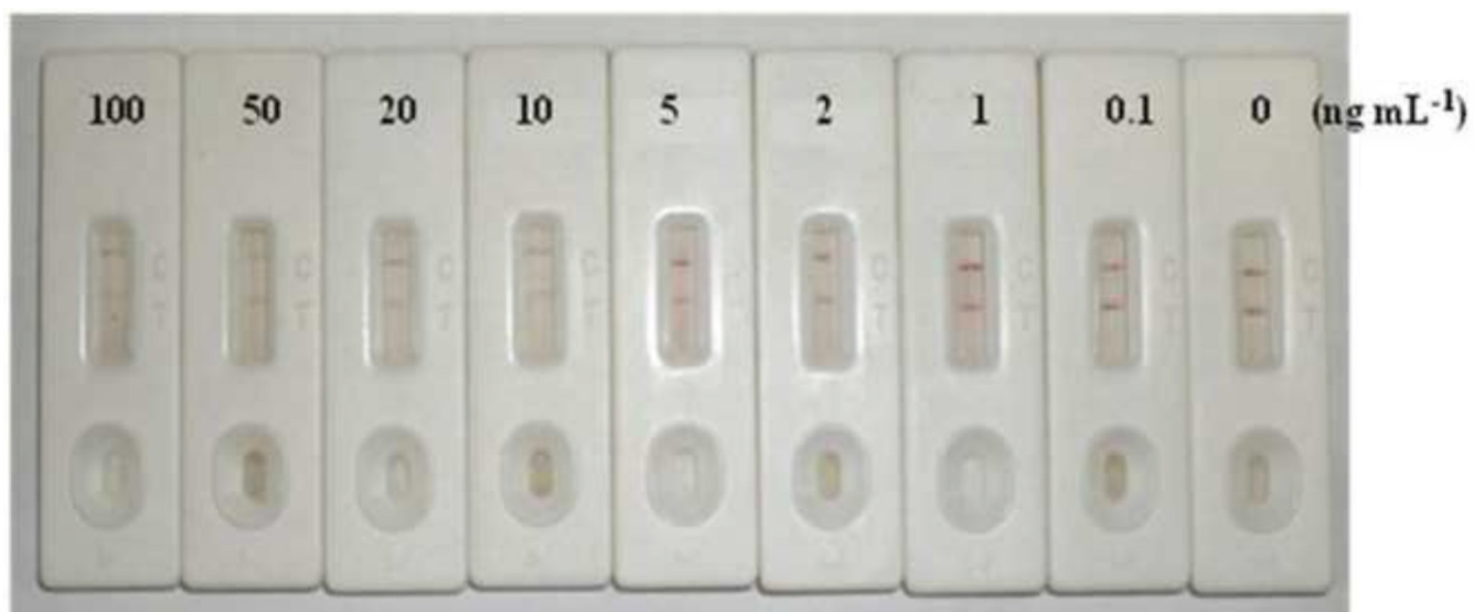
Fig. 5. Results of the lateral flow ICA for chlorpyrifos spiked into rice samples. Assay conditions were the same as those described in the legend of Fig. 4.
