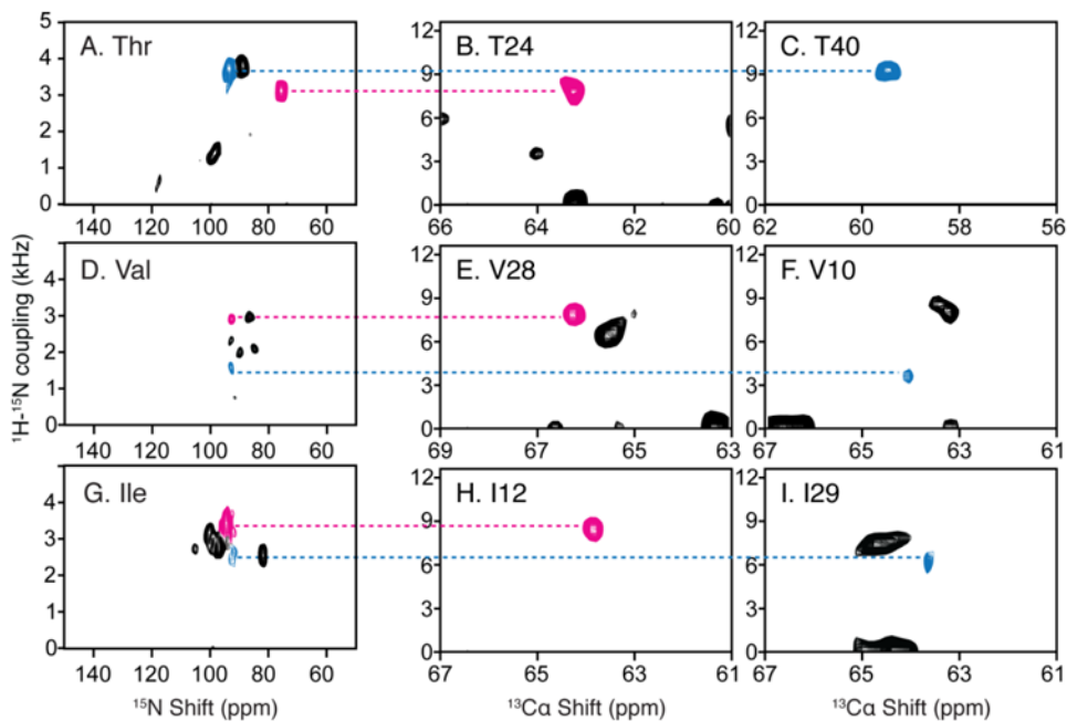
Fig. 5. Resonance assignments of residues in OS solid-state NMR spectra utilizing the ^1\text{H}-^{15}\text{N} dipolar couplings measured in RA MAS solid-state NMR experiments. A. D. and G. Two-dimensional SLF spectrum of amino-acid-type selectively ^{15}\text{N} labeled MerF in 'unflipped' DMPC/DHPC bicelles. B. C. E. F. H. and I. Two-dimensional SLF spectral planes extracted from a three-dimensional HnNCa experiment, of which the third dimension is ^{15}\text{N} chemical shift (Lu et al. 2013). The scales during aligning the ^1\text{H}-^{15}\text{N} dipolar couplings are adjusted for the scaling factors of the bicelles vs. liposomes (0.8) and of the alignment perpendicular to the magnetic field vs. rotational alignment parallel to the bilayer normal (0.5).
