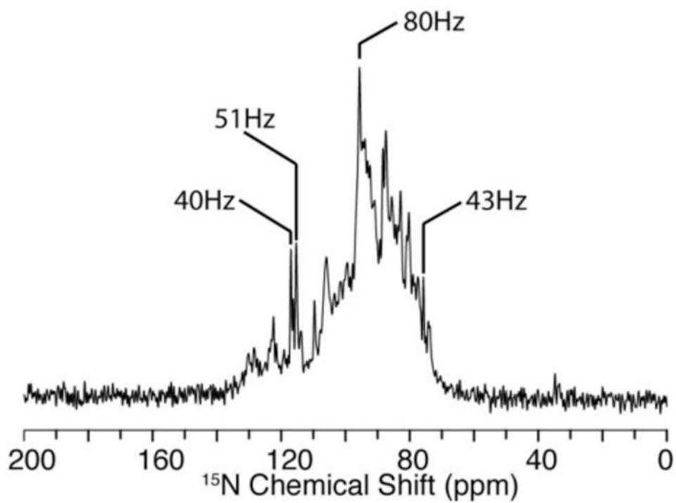
Fig. 1. ^{15}\text{N} solid-state NMR spectrum of uniformly ^{15}\text{N} labeled full-length MerF in q=3.2 14-O-PC/6-O-PC bicelles aligned with their normals perpendicular to the direction of the magnetic field. Line widths of selected resonances are marked in the figure.
