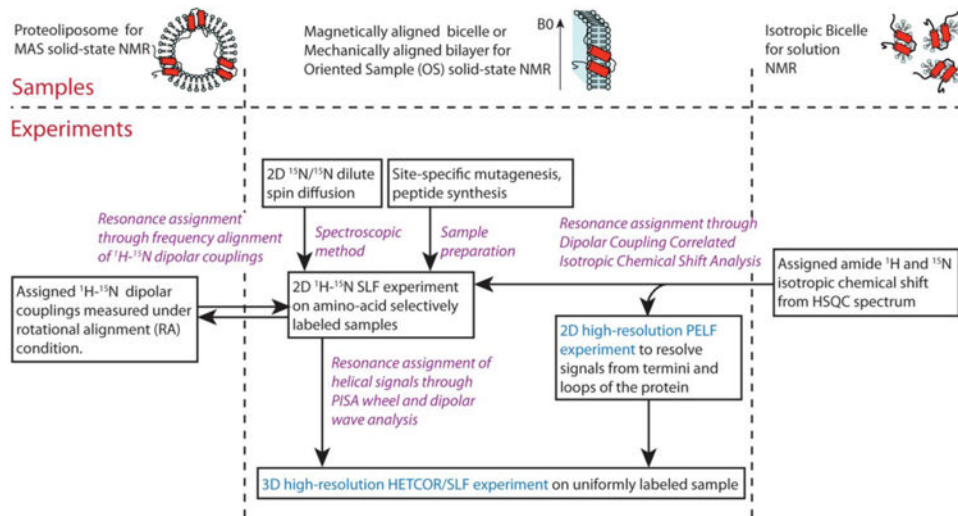
Fig. 7. A roadmap for resonance assignments of membrane protein samples in OS solid-state NMR. Purple highlights the five complementary resonance assignment methods. Cyan highlights the experiments with significantly improved resolution by new pulse sequences.
