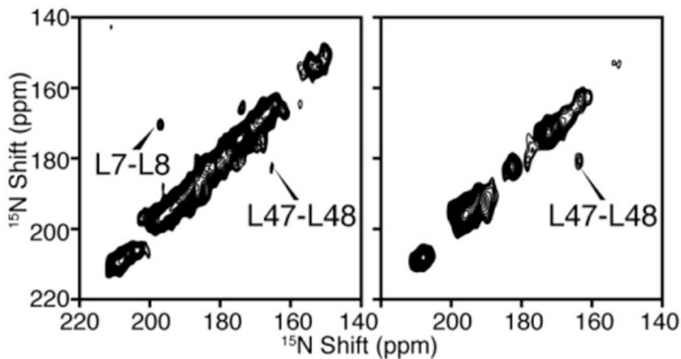
Fig. 6. Two-dimensional ^{15}\text{N}/^{15}\text{N} dilute spin exchange spectra of selectively ^{15}\text{N} -Leu labeled MerF in DMPC/DHPC bicelles aligned with their bilayer normal parallel to the magnetic field. A. Spectrum obtained using Mismatched Hartmann-Hahn (MMHH) spin diffusion (Nevzorov 2008). B. Spectrum obtained using Proton-driven Spin Diffusion (PDSD) (Cross et al. 1983).
