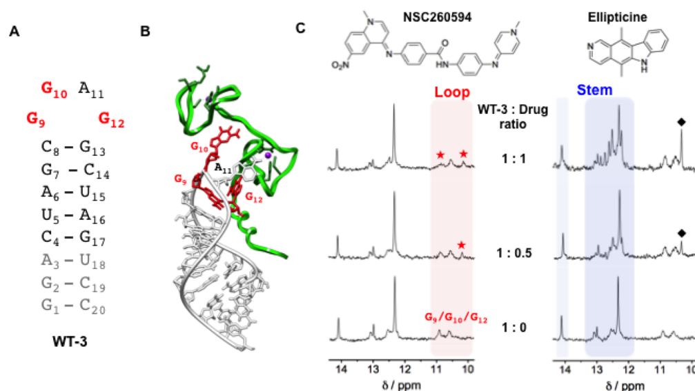
Figure 3. Interaction between the structural analogue of SL3 (WT-3) and the two small molecules, NSC260594 and ellipticine, as monitored by ^1\text{H} NMR. (A) Secondary structures of the WT-3 hairpin. In gray are reported the nucleotides added to SL3 in order to have a well-defined secondary structure suitable for NMR spectroscopy and in red the G9, G10, and G12 guanines constituting the tetraloop of SL3. (B) 3-D model of the HIV-1 nucleocapsid–WT-3 complex (PDB 1A1T) depicting the protein and the RNA hairpin with a green and white ribbon, respectively. The G9, G10, and G12 guanines essential for binding to the HIV-1 nucleocapsid are represented in red. (C) WT-3 ^1\text{H} NMR titration experiments with an increasing amount of the compounds NSC260594 and ellipticine. The imino protons between 12 and 14.5 ppm (blue region) are attributed to the Watson–Crick H-bonded base pairs of the stem of the hairpin structure and imino protons between 10 and 11 ppm (red region) are attributed to the WT-3 loop G bases. Red stars (★) highlight the alteration of the G9, G10, and G12 imino signals, and black diamonds (◆) highlight peaks attributed to ellipticine.
