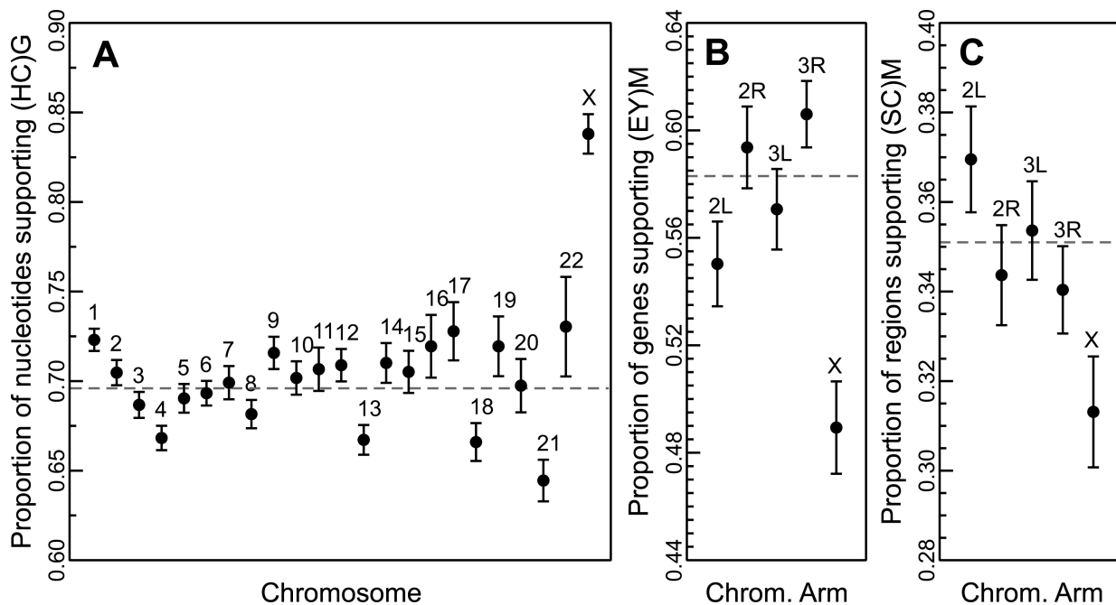
Figure 3. X-linked regions in the HCG alignment (A) show markedly increased support for the putative species tree over the autosomal average (dashed line). However, X-linked genes in the Dmel clade (B) and X-linked regions in the Dsim clade (C) show decreased support relative to autosomes.
