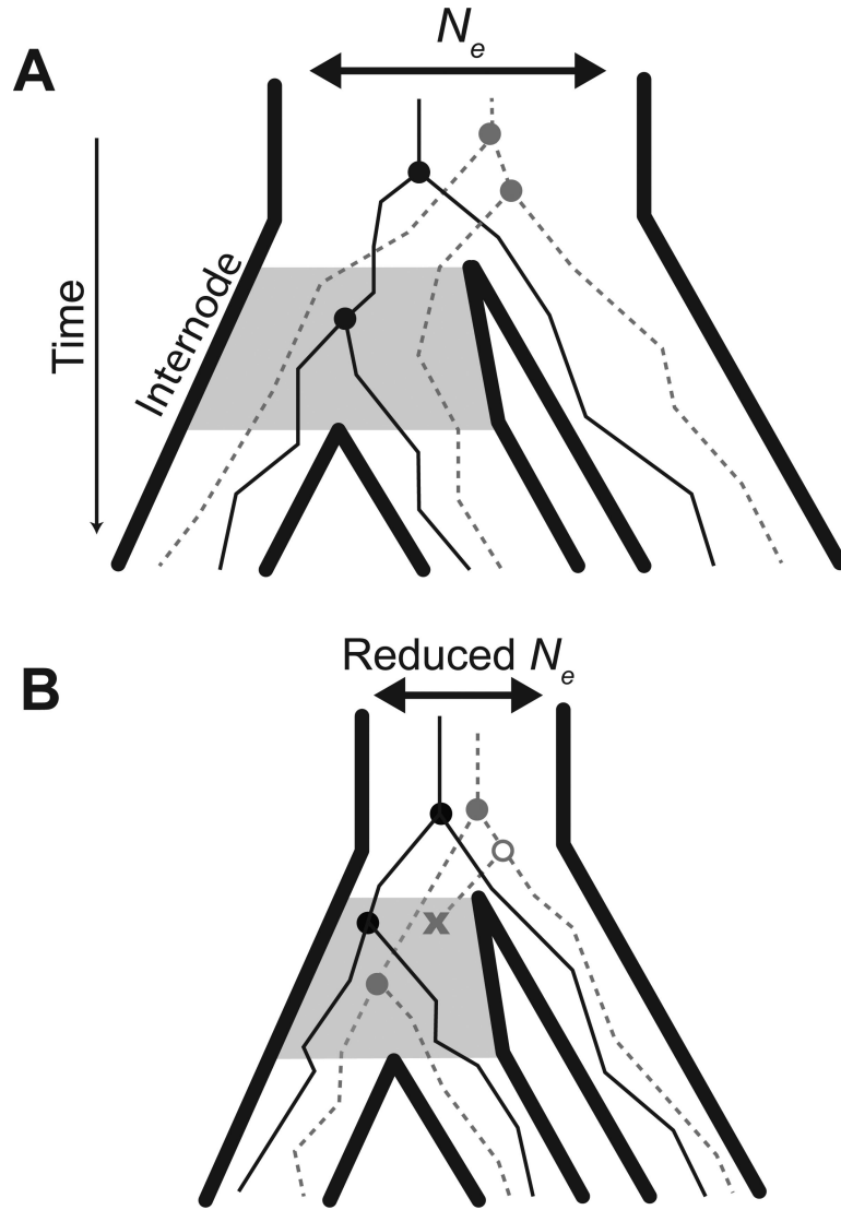
Figure 1. Species phylogeny (solid outline) in relation to gene trees (thin internal lines). Concordant gene trees have the same topology as the species tree (solid black line). When the effective population size ( N_e ) is large (A) and the internode time (shaded area) is short, lineages may not coalesce in the internode ancestral population and could lead to a discordant gene tree (dotted grey line). When N_e is reduced (B) lower levels of polymorphism are maintained in the internode population, and lineages are more likely to go extinct (x), decreasing the likelihood of sampling incongruent gene trees.
