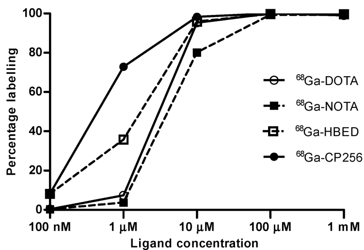
Fig. 2. Radiolabelling yield versus ligand concentration for ^{68}\text{Ga} -DOTA (pH 4.4, 30 min, 100 °C), ^{68}\text{Ga} -NOTA (pH 3.6, 10 min, room temp), ^{68}\text{Ga} -HBED (pH 4.6, 10 min, room temp) and ^{68}\text{Ga} -CP256, (pH 6.5, 5 min, room temp). All experiments were conducted with the same batch of ^{68}\text{Ga} eluate. All radiolabelling buffers were 0.2 M acetic acid/sodium acetate.
