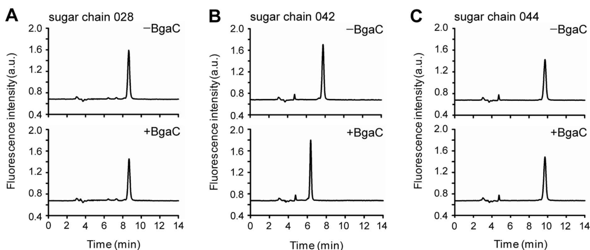
Figure 3 | HPLC analyses for hydrolysis products of polysaccharides by S. suis BgaC enzyme. (A). HPLC profile of PA-labeled sugar chain 028 with or without treatment of the recombinant S. suis BgaC protein. (B). HPLC test of PA-labeled sugar chain 042 following the S. suis BgaC protein-mediated hydrolysis. (C). HPLC assay for PA-labeled sugar chain 044 after the hydrolysis by the S. suis BgaC \beta -galactosidase. Minus: without addition of the BgaC protein; plus: addition of the BgaC protein. Designations: a.u., arbitrary units.
