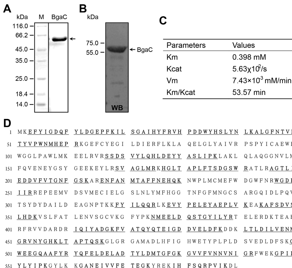
Figure 2 | Purification, identification and enzymatic characterization of the recombinant BgaC protein. (A). 12% SDS-PAGE profile of the purified BgaC protein of S. suis . The expected protein is indicated with an arrow. “M” is the abbreviation for protein molecular weight. The numbers on left hand represent protein size (kDa). (B). Western blotting analyses for the recombinant BgaC protein. (C). Enzymatic parameters determined for the BgaC \beta -galactosidase. The protocol used to measure the activity of \beta -galactosidase is found in section of Materials and Methods. Designations: Km, Michaelis constant; Vm, The maximum rate; Kcat: a rate constant. (D). MS-based identification of the recombinant BgaC protein. The tryptic peptides identified to match the BgaC sequence are given in underlined type.
