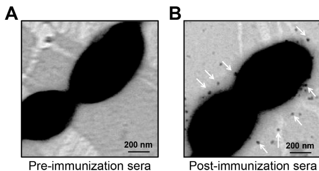
Figure 5 | Immune electron microscopy-based analyses of the BgaC protein. The BgaC protein is visualized to display on bacterial cell surface of S. suis 2 using the post-immunization sera ( Panel B ), whereas not using the pre-immunization sera ( Panel A ).
