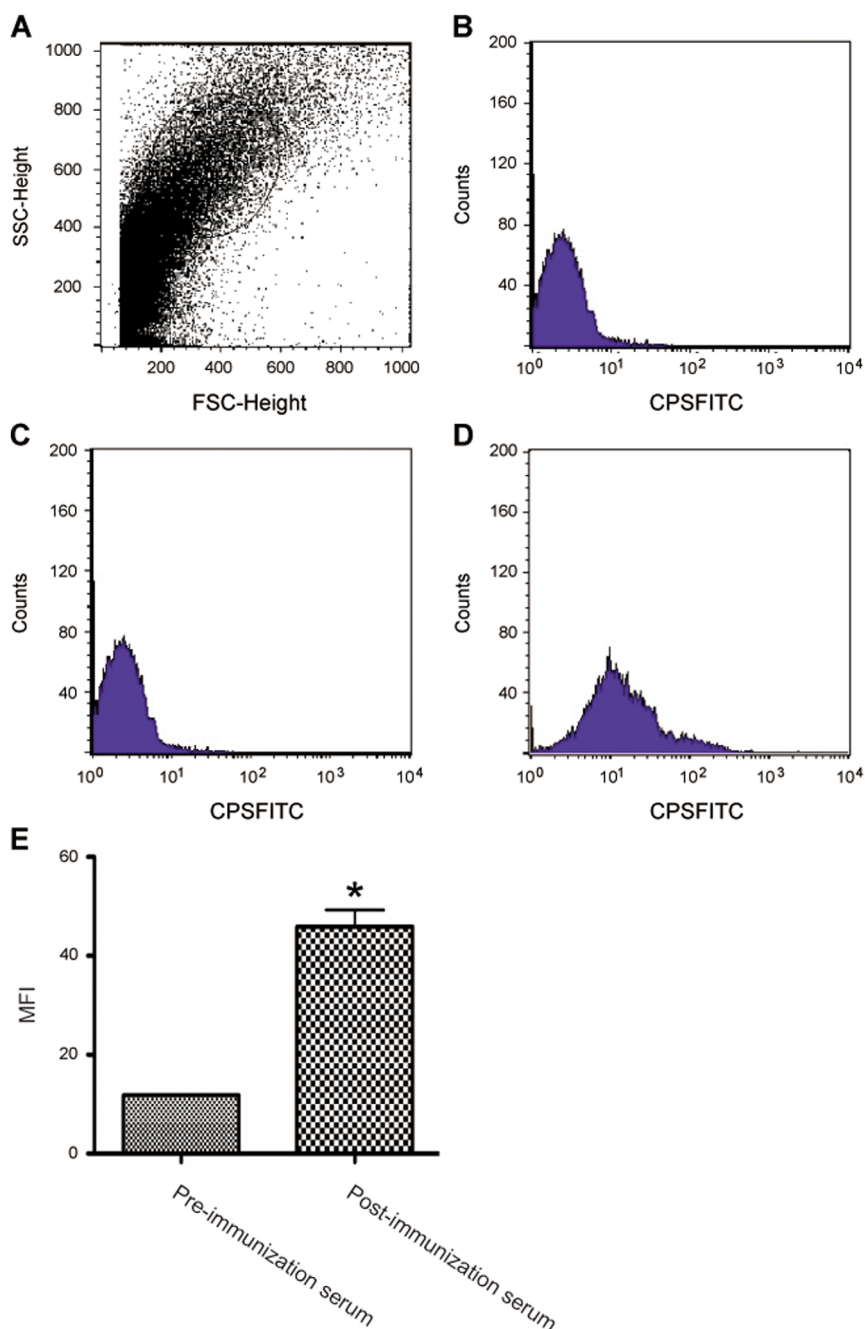
Figure 4 | Surface localization of the S. suis BgaC protein. (A). which suggests that the unlabeled bacteria can form a group suitable for fluorescence-activated cell sorting (FACS)-base analyses. (B). Mean fluorescence intensity (MFI) of the unlabeled bacteria. (C). MFI of S. suis treated with mouse pre-immune sera. (D). MFI of S. suis treated with mouse anti-BgaC sera. (E). Contrasting MFI of S. suis treated with mouse anti-BgaC sera (Panel D) to that with treatment of pre-immune sera (Panel C). Statistical analyses were performed by using a Student t test. *P-value was <0.05.
