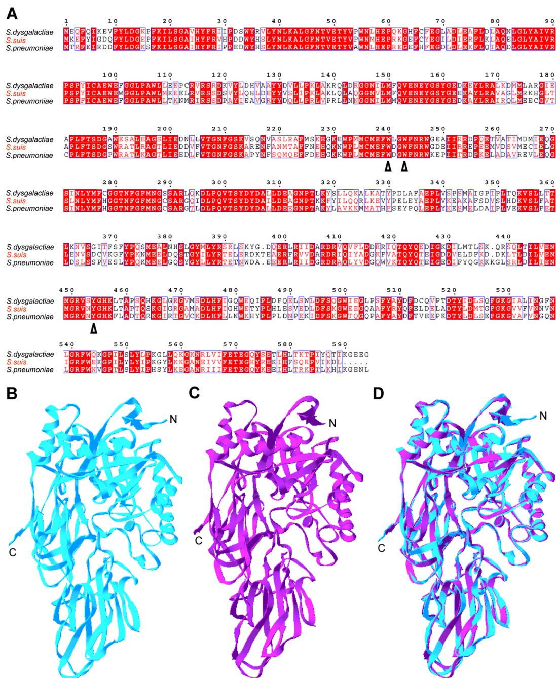
Figure 1 | Bioinformatics analyses of the BgaC proteins. (A). Multiple sequence alignments of BgaC homologues from three Streptococcus species. The amino acid sequences of three BgaC proteins used here are derived from S. pneumoniae (ABJ55509), S. suis 05ZYH33 (YP_001197815.1), and S. dysgalactiae (CC162219.1), respectively. Identical residues are indicated with white letters on a red background, similar residues are red letters on white, varied residues are in black letters, and dots represent missing residues. Three residues that are critical for enzymatic activity (240W, 243W & 454Y) are highlighted with arrows. (B). Ribbon representation of the known structure of S. pneumoniae BgaC protein. (C). The modelled structure of S. suis BgaC homologue. (D). Structure superposition of S. suis BgaC with the counterpart of S. pneumoniae . The structure of S. pneumoniae BgaC (PDB: 4E8D) is in blue, whereas that of S. suis BgaC is in purple. Designations: N, N-terminus; C, C-terminus.
