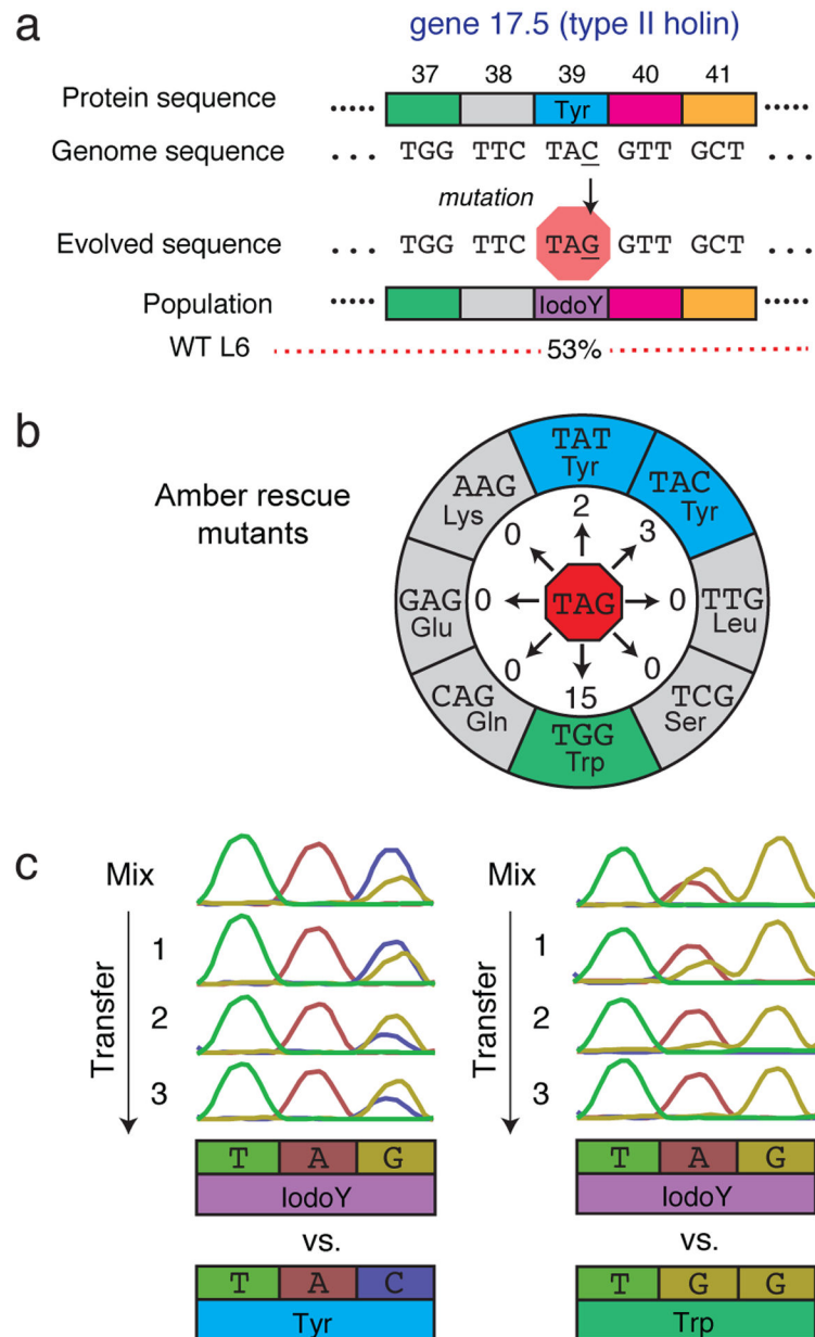
Figure 2. Beneficial amber mutation in the T7 holin II protein
