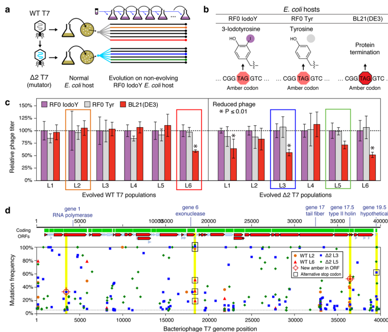
Figure 1. Genome evolution of a bacterial virus with a newly expanded genetic code
