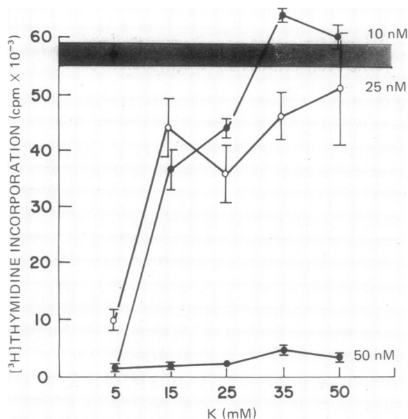
FIG. 3. Effect of increasing the \text{K}^+ concentration of external medium on [^3\text{H}] thymidine incorporation at 72 hr for lymphocytes cultured in the presence of three concentrations of valinomycin (50 nM, 25 nM, and 10 nM). Each point equals mean \pm SEM of triplicate cultures of a representative experiment.
