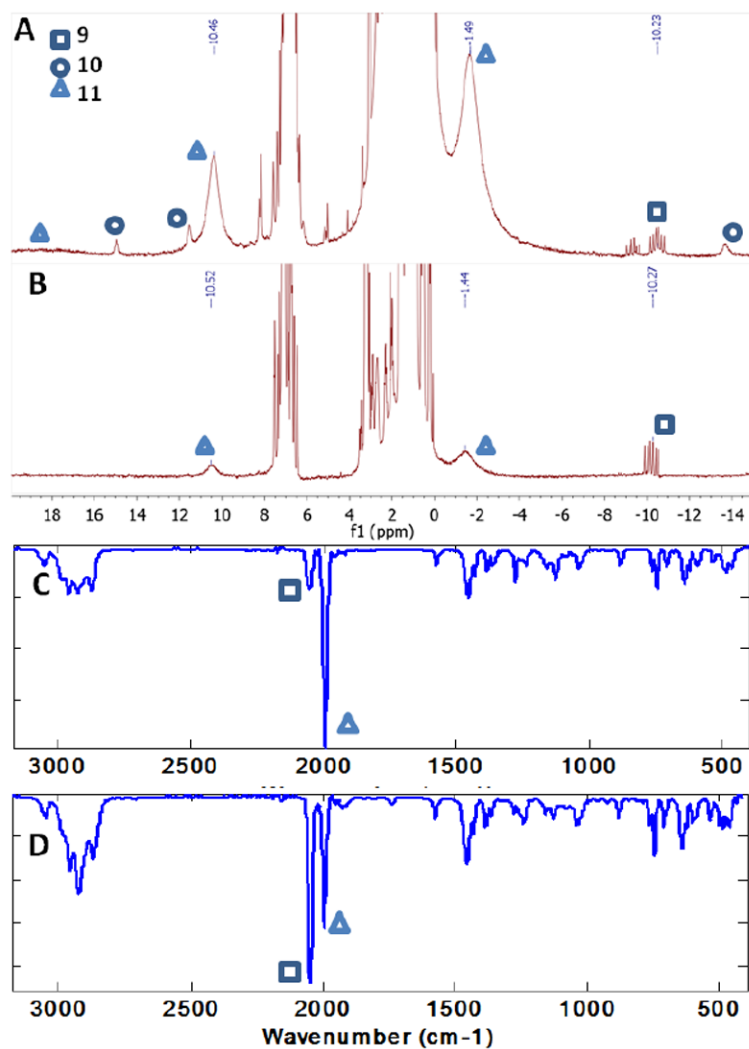
Figure 7. Spectroscopic analyses of reaction mixtures following the catalytic production of \text{NH}_3 using 12[\text{K}(\text{Et}_2\text{O})_{0.5}] as a catalyst. Symbols indicate characteristic resonances attributed to 9 , 10 , and 11 . (A),(C) ^1\text{H} NMR and IR spectra of a post-catalytic reaction mixture using 10 equiv. of [\text{H}(\text{Et}_2\text{O})_2][\text{BARF}_4] and 12 equiv. of \text{KC}_8 . (B),(D) ^1\text{H} NMR and IR spectra of a post-catalytic reaction mixture using 38 equiv. of [\text{H}(\text{Et}_2\text{O})_2][\text{BARF}_4] and 40 equiv. of \text{KC}_8 .
