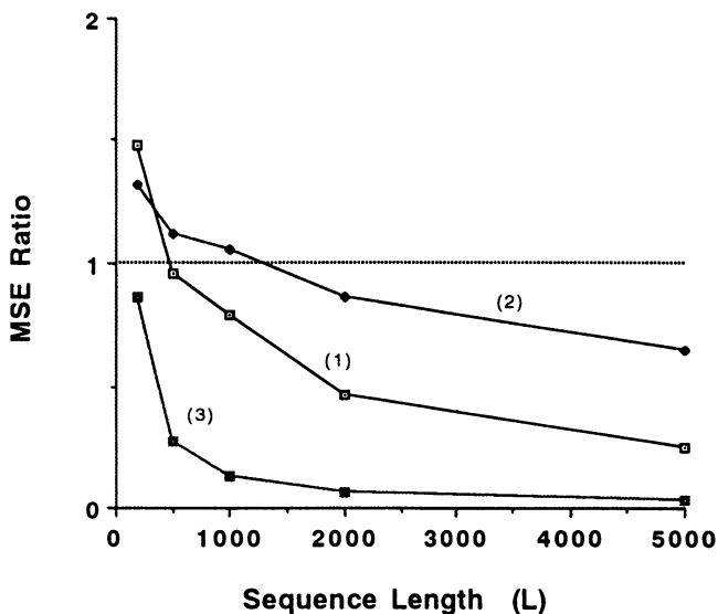
FIG. 1. Mean square error (MSE) ratios for SR/JC (curve 1), SR/TmN (curve 2), and SRV/SR (curve 3), plotted against the sequence length [JC, Jukes and Cantor's method (3); TmN, Tamura and Nei's method (5)]. The simulation model is SR for curves 1 and 2, but SRV for curve 3. The SR model is the same as that in Table 2. The SRV model is the same as the SR model except the rate varies among sites according to a gamma distribution with \alpha = 1 . The expected number of nucleotide substitutions is K = 0.5 . The number of replications is 1000.
