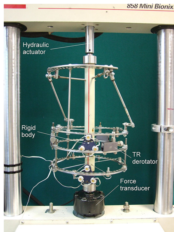
FIGURE 1. Ilizarov external fixator installed in the loading system.
