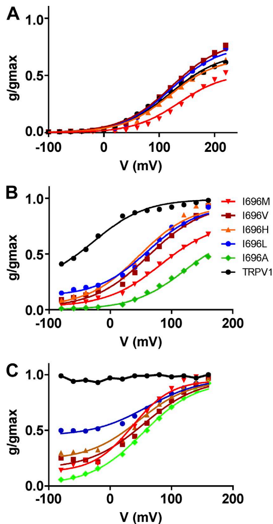
Figure 8. The proposed allosteric model reproduces the experimental data of TRPV1 wild type and I696X mutants. The figure depicts the normalized g - V curves obtained for the I696X mutants in the absence (A) and presence of capsaicin at 1 \mu M (B) and 100 \mu M (C). Solid lines depict the best fit to the allosteric model. Normalized g - V curves in the absence of capsaicin were fitted to Eq. 1, and results are given in Table 3. Normalized g - V curves in the presence of capsaicin were fitted to Eq. 3, fixing the values for the equilibrium constants obtained in the absence of capsaicin: J_o = 0.021 , L = 5.0 \times 10^{-4} , K_d = 10^{-5} , and z_g = 0.6 . The value of E given by the analysis was virtually 1 and, therefore, was kept constant to this value. The values obtained for allosteric constants P and D and free energy are depicted in Table 4.
