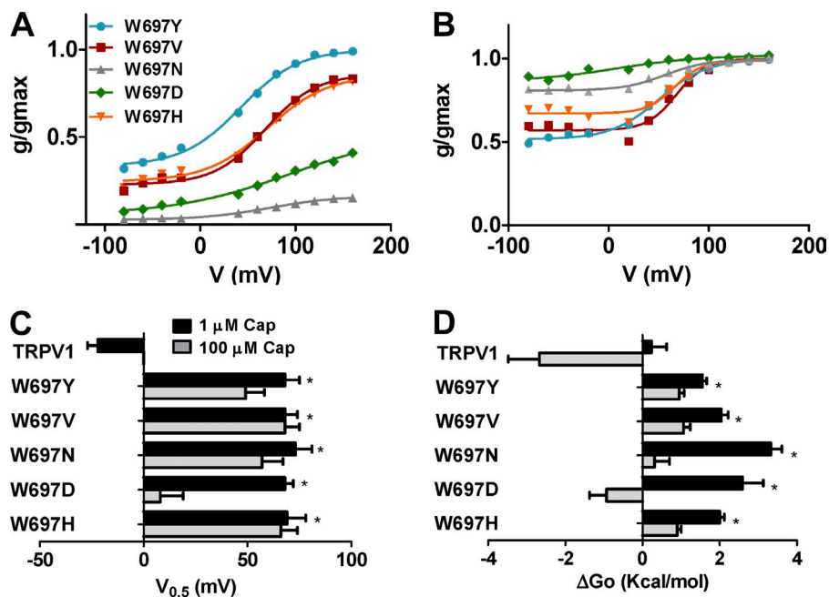
Figure 6. Mutation of W697 alters the response to capsaicin and voltage. (A and B) Normalized g - V relationships for selected W697X mutants in the presence of 1 \mu M (A) and 100 \mu M (B) capsaicin. Solid smooth lines depict the best fit to a Boltzmann distribution to obtain the V_{0.5} and z_g values. (C) V_{0.5} values of the different W697X mutants obtained from the g - V curves. (D) \Delta G_o values obtained as the sum of the voltage dependent components at 0 mV ( \Delta G_o(V) ) and independent ( \Delta G_o(I) ) components considering a simple two-state model between a closed and open state. g - V curves were normalized with respect to the true g_{max} of the channel obtained in the presence of 100 \mu M capsaicin (Tables 1 and 2). Data are given as mean \pm SEM (error bars), with n (number of cells) \geq 5. *, P < 0.05 as compared with wild type, using the nonparametric Wilcoxon test.
