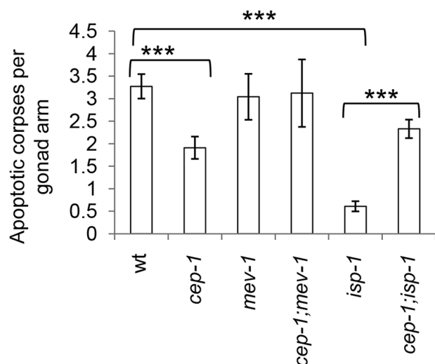
Figure 2. CEP-1 mediates reduced physiological germline apoptosis in the isp-1 mutant. Physiological levels of apoptosis were quantified by counting the number of apoptotic corpses per gonad arm in various C. elegans strains. The corpses were counted using DIC microscopy at 63 \times magnification 48 hr post L4. The data represent the average of at least 3 independent experimental replicates ( n \geq 15 gonad arms for each) \pm standard error. Statistical analysis was done using the Mann-Whitney U-test. *** p < 0.001 . doi:10.1371/journal.pgen.1004097.g002
