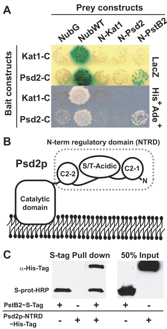
FIGURE 2. PstB2p and Psd2p form a complex. A , mbSUS was used to test for interactions between Psd2p and PstB2p in vivo . NubG, NubWT, and Cub refer to the C-terminal or N-terminal halves of ubiquitin, as described under “Results.” Kat1, a K + channel from Arabidopsis , serves as an irrelevant protein negative control for both bait and prey proteins. NubG and NubWT serve as negative and positive controls for bait protein stability and expression, respectively. B , Psd2 is a modular protein and contains two C2 domains separated by a large acidic, hydrophilic tract. This region of the protein, referred to as the NTRD, is not present in mitochondrial or bacterial PSD enzymes and contains domains essential for the transport functions of Psd2p. C , protein affinity assays were conducted using the S-tagged PstB2 protein and His-tagged Psd2-NTRD protein. The interaction of Psd2-NTRD with S-protein-agarose beads was dependent on the presence of S-tagged PstB2p.
