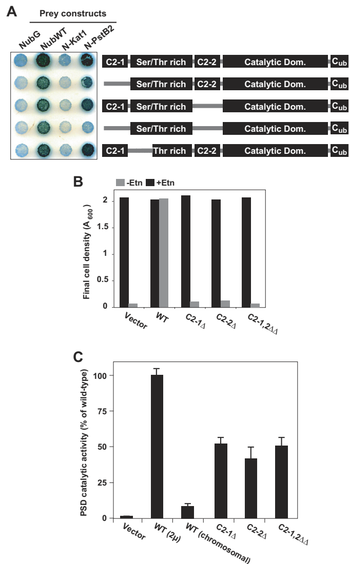
FIGURE 3. The C2 domains of the Psd2-NTRD are required for interaction with PstB2 and in vivo transport functions but not for catalytic activity. A, the mbSUS was used to assay the interactions between PstB2p and deletion mutants of the N-terminal regulatory domain of Psd2p (Psd2-NTRD). Schematic diagrams to the right of the interaction results show the sequence fragment that was deleted. B, growth assays were conducted as described under “Results” and show that the C2-1 domain is required for growth when the function of Psd2p is essential. C, transport-independent PSD assays of the Psd2p deletion mutants using NBD-PtdSer as the substrate were conducted according to previously described methods. Error bars, S.E. of three independent analyses conducted in duplicate.
