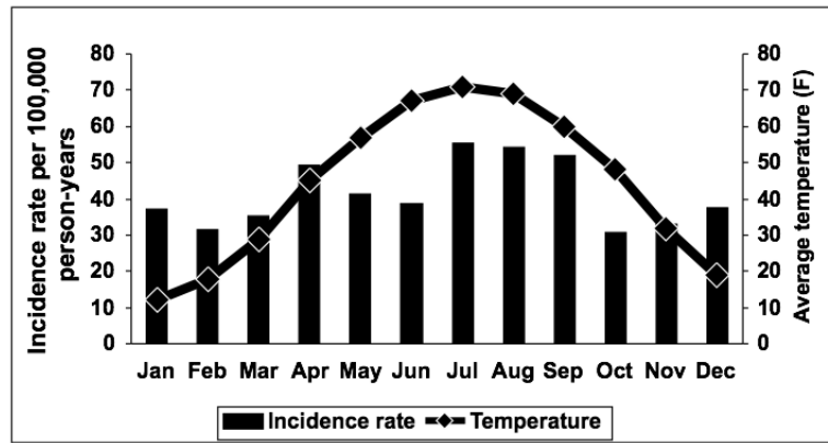
Figure 1. Monthly age- and gender-adjusted incidence rates of Escherichia coli bloodstream infection and average monthly temperatures, 1998-2007.
