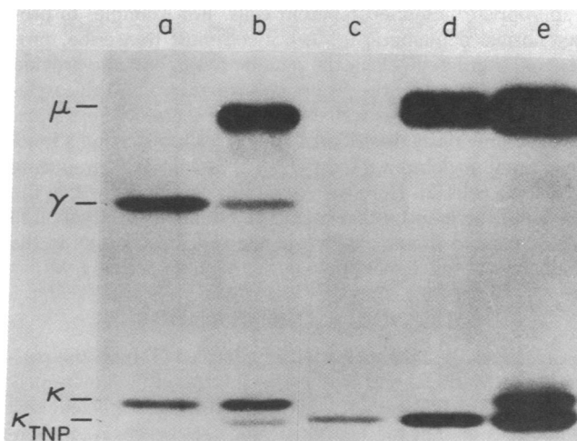
FIG. 2. Analysis of heavy and light chains of secreted Ig. G418-resistant transformant clones were biosynthetically radiolabeled with [ ^{14} C]leucine as described (7). Secreted immunoglobulins were immunoprecipitated with rabbit anti-mouse IgM antibody complexed with protein A-Sepharose CL-4B beads (Pharmacia). The precipitated material was reduced with 2-mercaptoethanol and analyzed by electrophoresis on a NaDodSO _4 /polyacrylamide gel. Lane a, X63Ag8; lane b, XR19L4; lane c, igm-10; lane d, IR44L1; and lane e, wild-type hybridoma Sp603.
