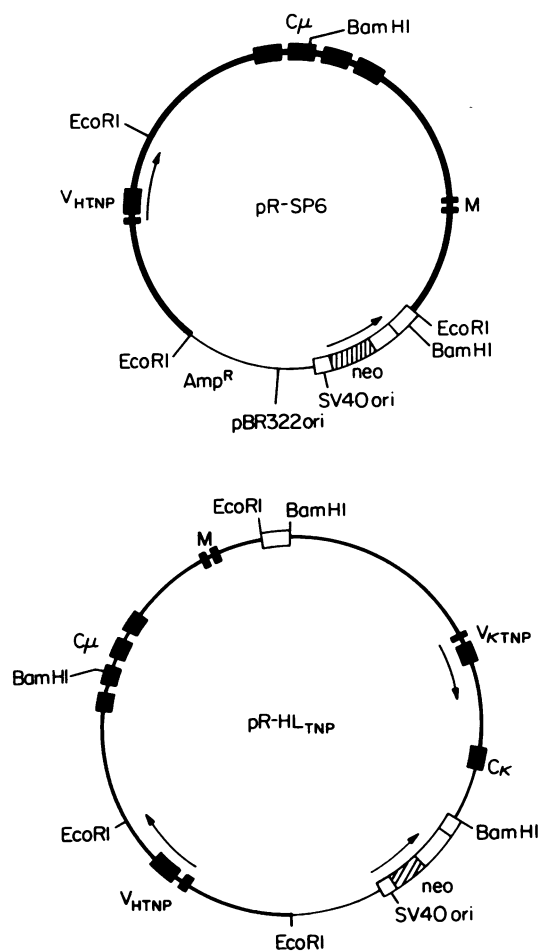
FIG. 1. Structure of the pR-Sp6 and pR-HL _{\text{TNP}} plasmids. pR-Sp6 contains the functionally rearranged \mu_{\text{TNP}} gene ( \approx 16 kbp), which was inserted into the Eco RI site of pSV2- neo (see text). In addition to the \mu_{\text{TNP}} gene, pRHL _{\text{TNP}} contains the functionally rearranged \kappa_{\text{TNP}} gene (9.6 kbp) at the Bam HI site (2). Ig genes are represented by heavy dark lines. The directions of transcription of the Ig genes and the SV40 early region are indicated by arrows. The \mu and \kappa exons are shown as filled boxes. M denotes alternative COOH-terminal coding regions that are utilized in the synthesis of membrane IgM. Thin lines are of pBR322 origin. The white boxes denote DNA derived from SV40, into which the bacterial gene conferring neomycin resistance (hatched box) has been inserted. For specific details concerning the pSV2- neo transfer vector (donated by P. Berg), see ref. 17.
