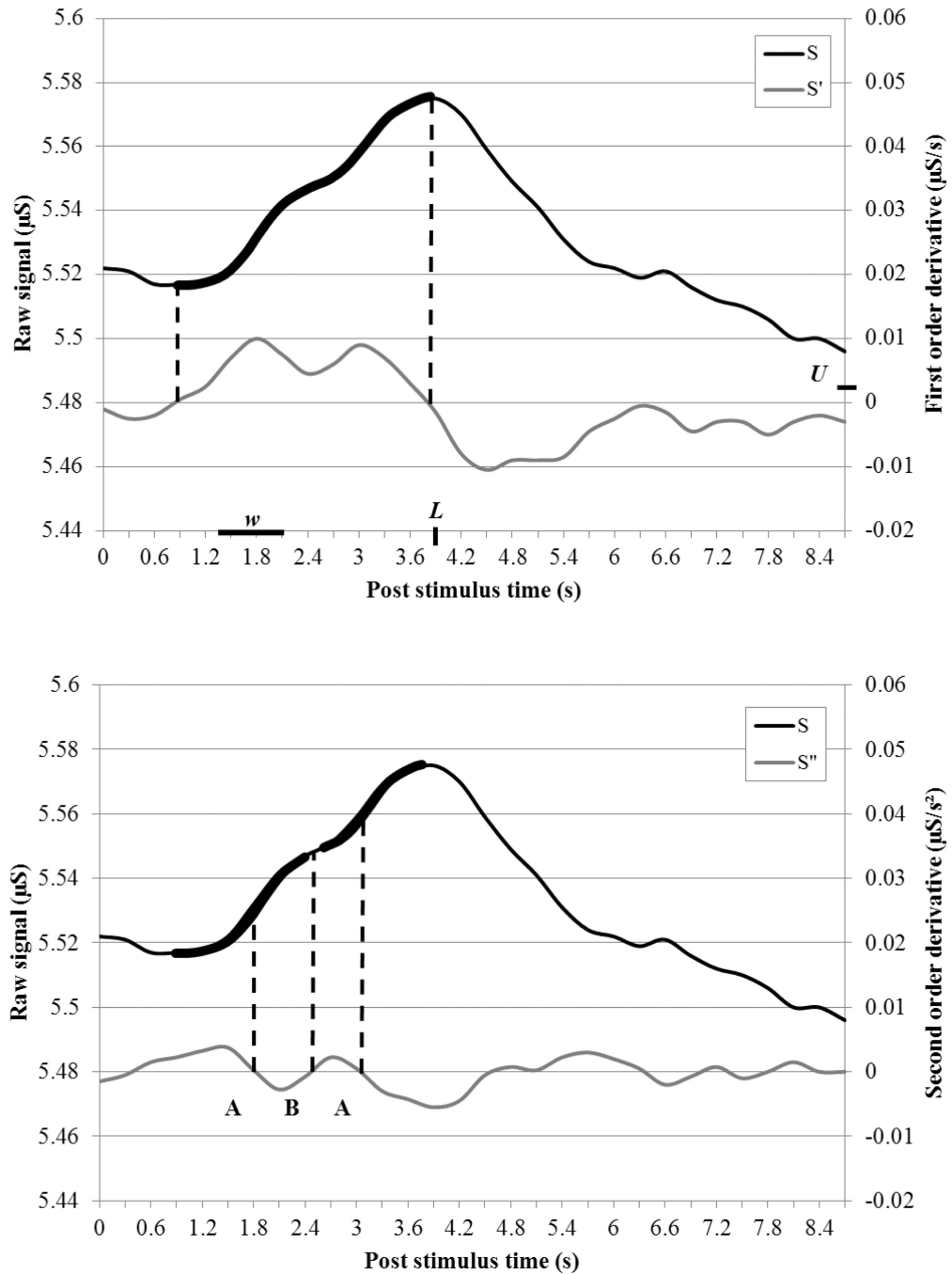
Figure 1. Example of Autonomate's SCR amplitude estimation with overlapping responses (A) Candidate SCR is detected by examining the first order temporal derivative S' up to time L for contiguous sections above threshold U \mu\text{S/s} for at least w s. (B) Candidate SCR is split by finding a sequence of zero crossings in second order temporal derivative S'' . Crossings where S' is increasing are labeled A and crossings where S' is decreasing are labeled B . A pattern of A-B-A crossings indicates an inflection point where a candidate SCR should be split at point B . Candidate SCRs are indicated with thick black line superimposed on raw skin conductance signal S . Zero crossings are indicated with dashed lines.
