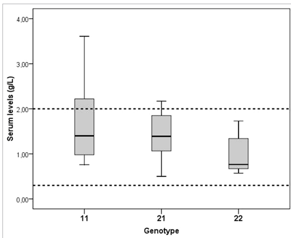
Figure 3. Haptoglobin serum levels in healthy controls for each HP genotype. Values represent medians (lines) with their quartiles (upper and lower level box).
