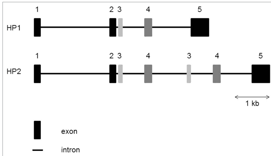
Figure 1. Structure of the human HP gene. The human HP2 allele arose by duplication of exons 3 and 4 of the HP1 allele. HP, Haptoglobin; kb, kilobase
