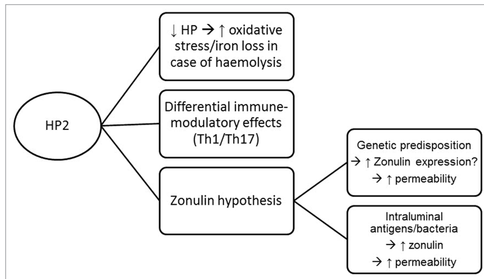
Figure 4. Summary diagram of the different ways HP(2) can be involved in IBD pathogenesis. HP, Haptoglobin.
