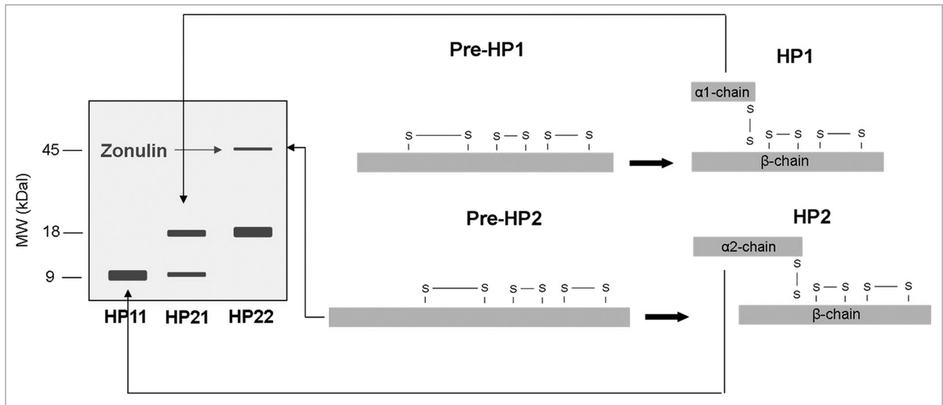
Figure 2. The structure of pre-HP1 and pre-HP2, and HP1 and HP2 is depicted on the right. It is also shown how the different proteins can be visualized on western blot (left side). (Adapted from 8 ). HP, Haptoglobin; MW, molecular weight; kDa, kilo dalton.
