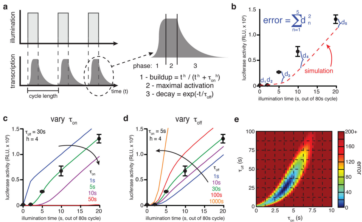
Figure 3. Kinetic modeling of VP-EL222 activation
