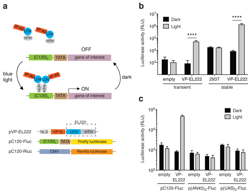
Figure 1. Model for the EL222-based light-inducible gene expression system
