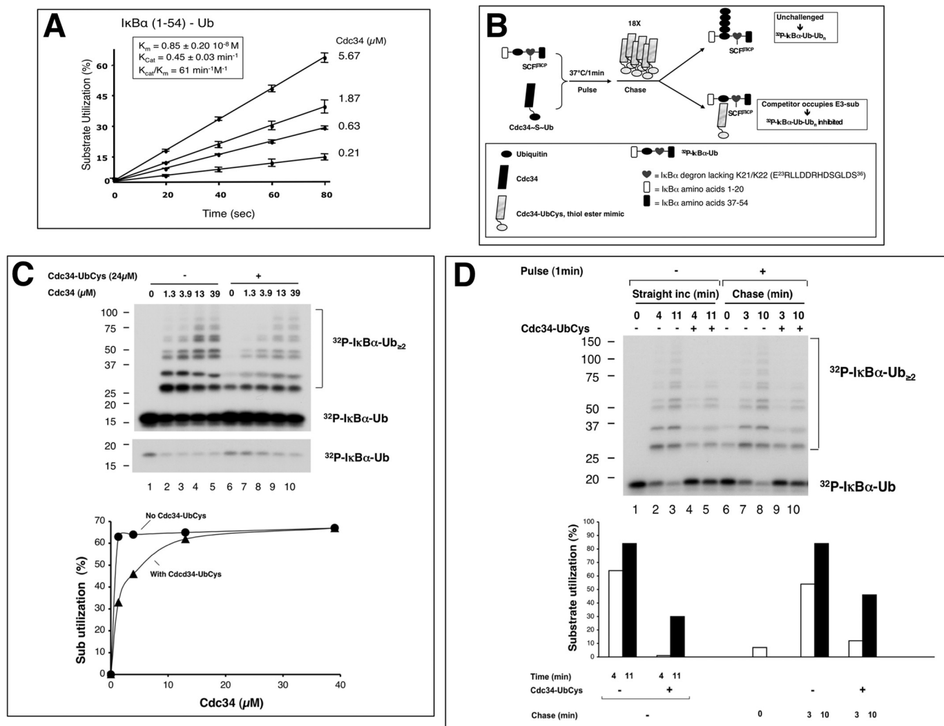
FIGURE 3. Dynamic association between Cdc34 and the SCF βTrCP1 -IκBα-Ub complex. A , kinetic parameters of polyubiquitination of IκBα(1-54)-Ub by SCF βTrCP2 and Cdc34. 32 P-labeled IκBα(1-54)-Ub (2 pmol) was incubated with SCF βTrCP2 (~2 pmol) for 10 min. Separate mixtures of Cdc34~Ub at differing concentrations (5.67, 1.87, 0.63, and 0.21 \mu\text{M} ) of Cdc34 were incubated at 37 °C for 5 min. The two mixtures were combined, and reactions were stopped by the addition of SDS-loading buffer after 20, 40, 60, or 80 s. Substrate utilization of three independent data sets was calculated and shown graphically. K_m and K_{\text{cat}} were estimated by fitting to Michaelis-Menten kinetics and shown in the inset box. B , the competition scheme. The detailed procedure is described under "Experimental Procedures." C , the inhibition of Cdc34-Ub Cys on Cdc34-catalyzed elongation of 32 P-IκBα-Ub. The inhibitory effects were reversed by high concentrations of Cdc34. A short exposure of the input substrate is shown to better reveal its reduction with reaction time. D , the competition reaction. The effects of Cdc34-Ub Cys , which was added after the reaction had been initiated, are shown. The substrate conversion was quantified and is shown graphically.
