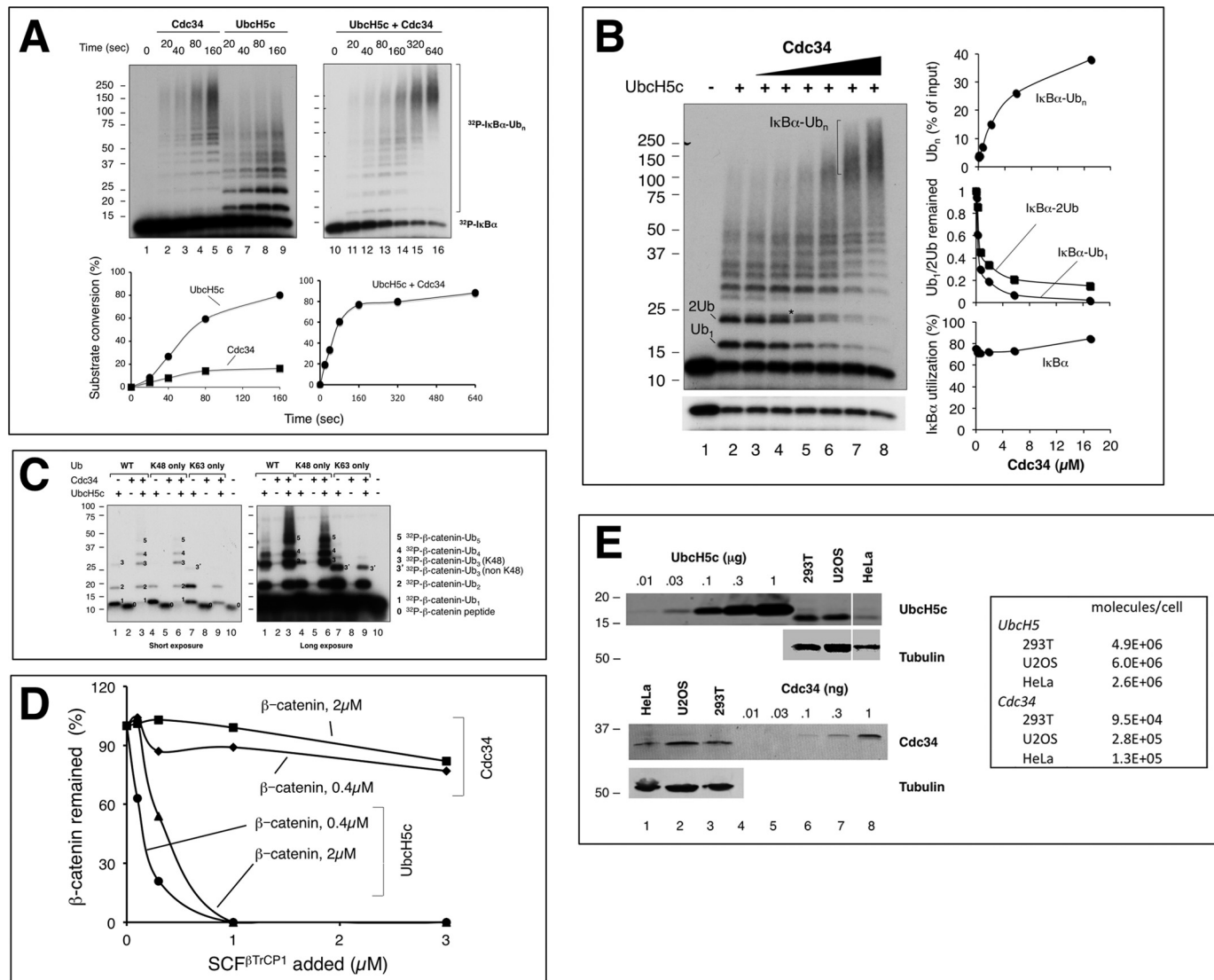
FIGURE 2. In vitro ubiquitination of I\kappa B\alpha and \beta -Catenin by SCF^{\beta TrCP2} , UbcH5c, and Cdc34. A , kinetic analysis of polyubiquitination of I\kappa B\alpha (1–54) by SCF^{\beta TrCP2} in the presence of UbcH5c, Cdc34, or both UbcH5c and Cdc34. Ubiquitination was carried out as described under “Experimental Procedures” with substrate (0.1 \mu M ), E3 (0.1 \mu M ), UbcH5c (17 \mu M ), and Cdc34 (17 \mu M ). B , effect of Cdc34 concentration on polyubiquitination of I\kappa B\alpha (1–54) by SCF^{\beta TrCP2} in the presence of UbcH5c. Ubiquitination was carried out as in panel A at 37°C for 3 min. Reaction products are marked on the gel. Although Ub_1 denotes mono-ubiquitinated I\kappa B\alpha (1–54) at either Lys-21 or Lys-22, 2Ub represents the di-Ub products with Ub conjugated at both Lys-21 and Lys-22. * refers to I\kappa B\alpha (1–54) attached with a di-Ub chain formed at either Lys-21 or Lys-22. C , combined actions of UbcH5c and Cdc34 drive polyubiquitination of \beta -catenin by SCF^{\beta TrCP2} . Ubiquitination was carried out as in panel A with the wild type Ub or variants as indicated at 37°C for 15 min. Both short and long exposures are shown. Substrate and reaction products are marked on the gel, with numbers denoting the number of Ub moieties. D , analysis of polyubiquitination of \beta -Catenin by SCF^{\beta TrCP1} with UbcH5c or Cdc34 in a range of concentrations of substrate or E3. Varying concentrations of \beta -catenin or SCF^{\beta TrCP1} , as indicated, were used for the ubiquitination assay. The results were quantified and are shown graphically. E , immunoblot analysis of cellular concentrations of UbcH5 and Cdc34. Protein extracts from the indicated cell lines were subject to immunoblot analysis along with purified UbcH5c and Cdc34 in amounts as indicated. For the immunoblots of UbcH5 or Cdc34, protein lysates derived from 300,000 or 150,000 cells, respectively, were used. The box indicates the estimated number of molecules for UbcH5 or Cdc34 in the indicated cell line.
