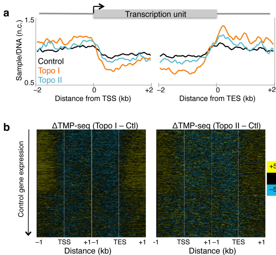
Figure 2. Topoisomerase inhibition increases torsional stress genome-wide
