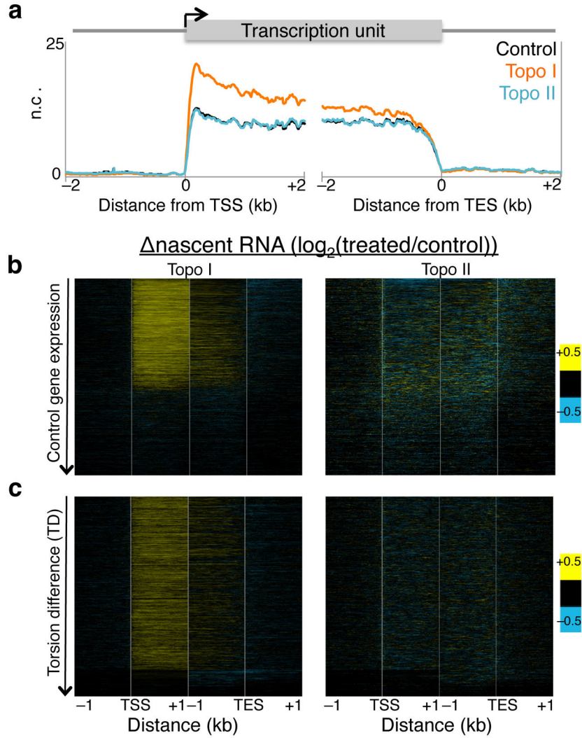
Figure 4. Altered Pol II elongation kinetics upon topoisomerase inhibition
