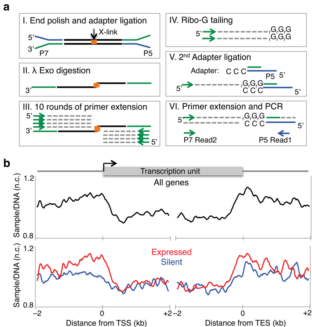
Figure 1. High resolution detection of supercoiling states
