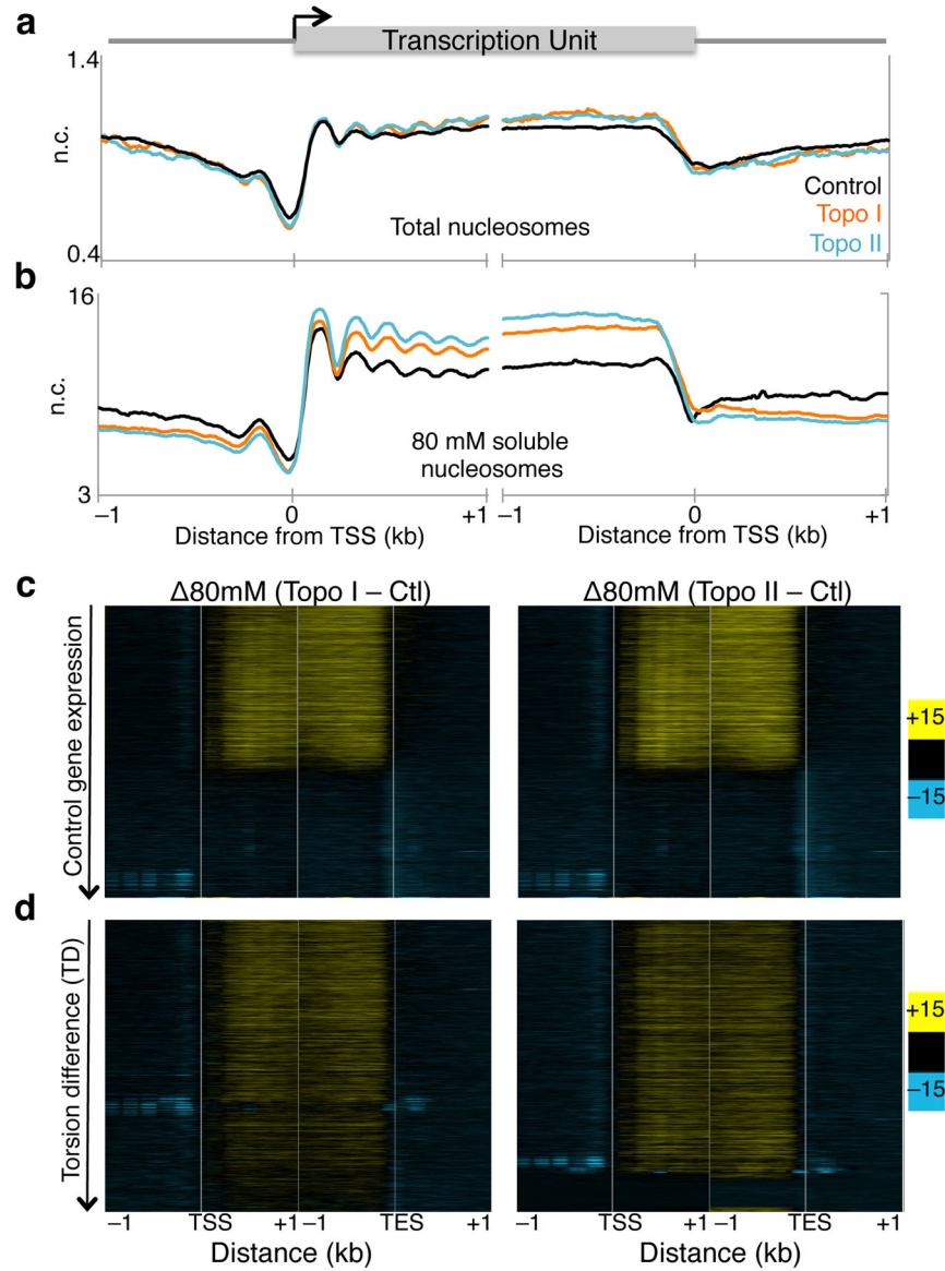
Figure 5. Topoisomerase inhibition affects low-salt chromatin fractionation (a) Two replicates of total MNase digested chromatin were sequenced from treated and untreated cells, and the average signal surrounding the transcription start site (TSS) and transcription end site (TES) in all genes for >120 bp reads were plotted. n.c. Normalized counts. (b) Sequenced reads from 80 mM salt soluble fraction for two replicates were mapped onto the genome and the average signals surrounding the TSS and TES were determined. (c) The difference in low-salt soluble signals between control and Topo I- (left), and II-inhibited (right) samples were determined and displayed as heat maps with genes ordered in decreasing expression in control samples for reads of length >120 bp. (d) Heat maps as in (b) arranged by decreasing TD. Contrast = 15.
