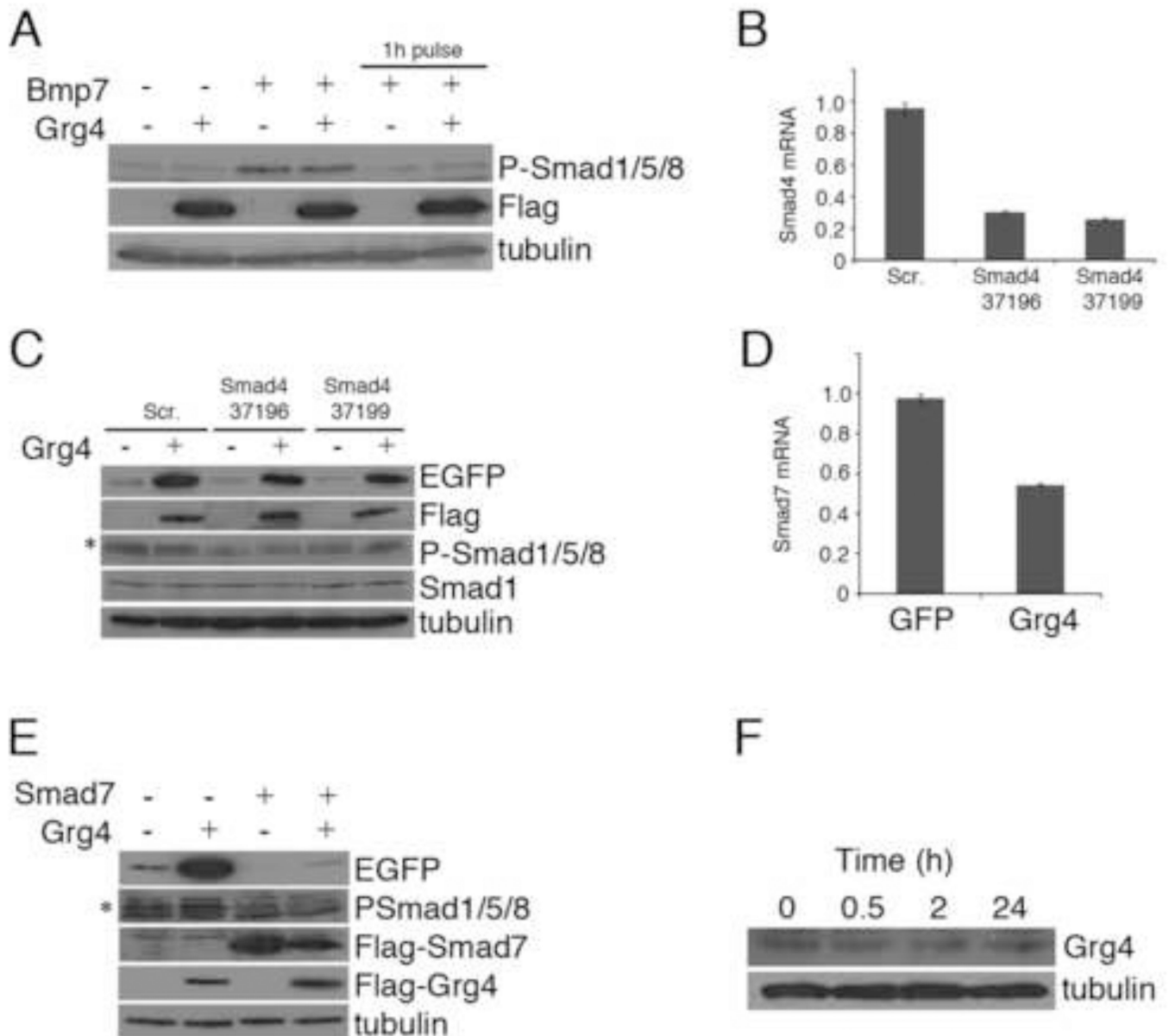
Figure 4. Grg4 mediated activation through inhibition of Smad7
