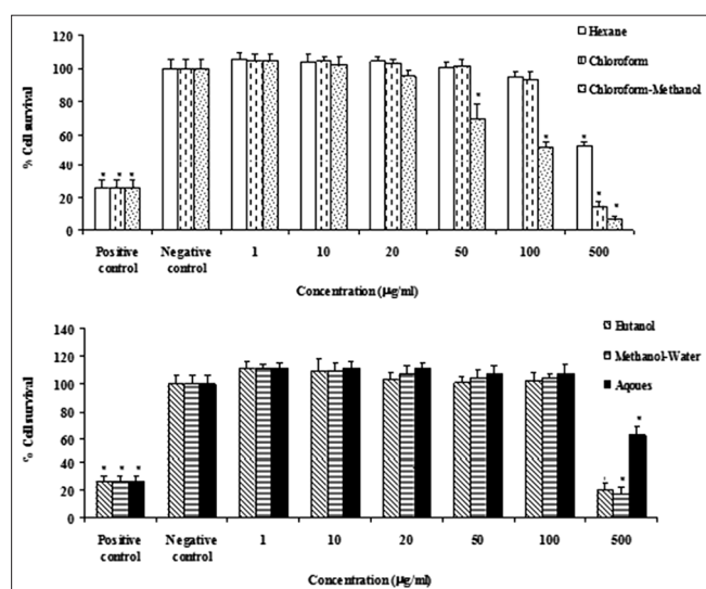
Figure 3: The effects of different extracts of Zizyphus spina-christi on Hela cells viability of the cells was determined by MTT assay. Percent cell survival in the control group was assumed 100. (a) hexane, chloroform and chloroform-methanol extracts. (b) Butanol, methanol-water and aqueous extracts. * = P < 0.05 , n = 3
