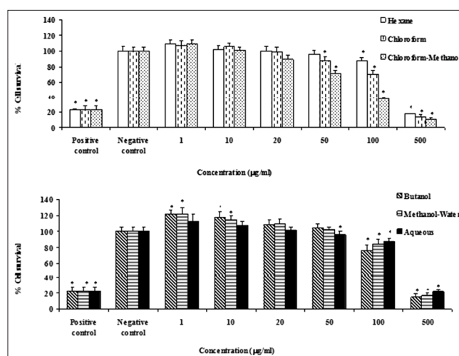
Figure 4: The effects of different extracts of Zizyphus spina-christi on MDA-MB-468 cells viability of the cells was determined by MTT assay. Percent cell survival in the control group was assumed 100. (a) hexane, chloroform and chloroform-methanol extracts. (b) Butanol, methanol-water and aqueous extracts. * = P < 0.05 , n = 3
