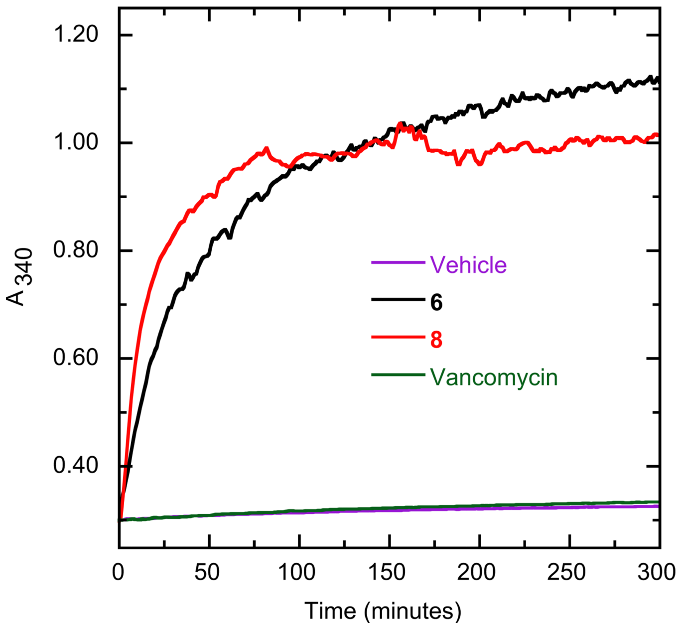
Fig. 2. Impact of select phenyl-naphthalenes on the polymerization of S. aureus FtsZ (SaFtsZ), as determined by monitoring time-dependent changes in absorbance at 340 nm ( A_{340} ). Polymerization profiles of SaFtsZ (10 \mu M) in the presence of DMSO vehicle (violet) or 40 \mu g/mL of either 6 (black), 8 (red), or the non-FtsZ-targeting comparator antibiotic vancomycin (green) are depicted.
