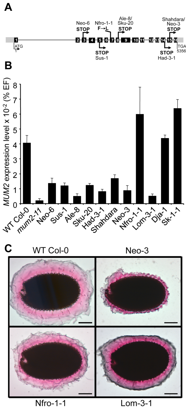
Figure 1. Characterization of natural mum2 mutants. (A) Schematic representation of the MUM2 gene indicating the positions of the causal mutations in the different accessions and their effect on the encoded protein in capital letters. Boxes represent exons; black shading shows coding sequence; grey shading indicates 5' and 3' untranslated regions. (B) Steady state MUM2 mRNA levels in developing siliques of indicated accessions, 8–12 days after pollination, represented as a percentage of the constitutive EF1α-4a (EF) gene abundance. Error bars represent SE (n=6). (C) Ruthenium red stained seeds of indicated accessions after forced mucilage release by sequential treatment with HCl and NaOH. WT, wild type. doi:10.1371/journal.pgen.1004221.g001
