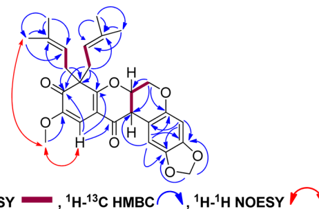
Figure 2. Selected NMR correlations of 1 .
