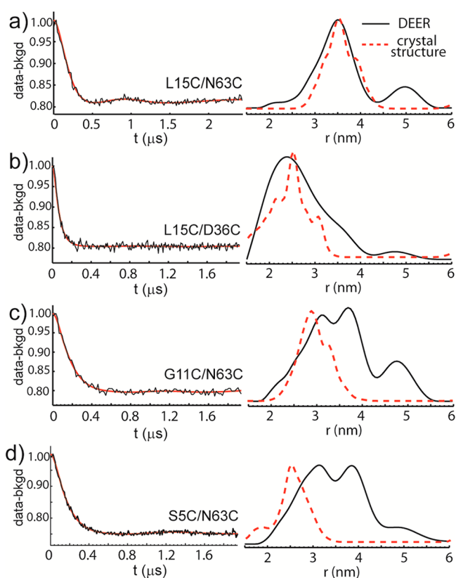
Figure 2. X-band DEER of spin-labeled MMOB double cysteine mutants in H_{ox} -2B complex and the corresponding distance distributions. Left panels, background subtracted DEER data (black) and simulated fits (red) for spin-labeled MMOB double mutants L15C/N63C, L15C/D36C, G11C/N63C, and S5C/N63C in H_{ox} -2B complex. Right panels, the corresponding distance distributions derived from the DEER data (black) and from the crystal structure of H_{ox} -2B complex (red dashed lines). DEER data were processed by using DeerAnalysis 2011. 16 The distance distributions derived from the crystal structure were modeled by using MMM program package 2011.2. 17
