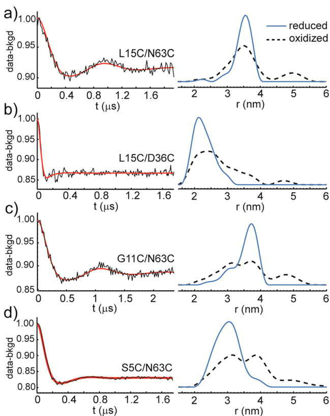
Figure 3. X-band DEER of spin-labeled MMOB double cysteine mutants in the H_{red} -2B complex and the corresponding core-to-tail distance distributions. Left panels, background subtracted DEER data (black) and simulated fits (red) for spin-labeled MMOB double mutants L15C/N63C, L15C/D36C, G11C/N63C, and S5C/N63C in the H_{red} -2B complex. Right panels, the corresponding distance distributions derived from the DEER data (blue); the DEER derived distance distributions of the corresponding H_{ox} -2B complex are also shown (black dashed lines). DEER data were processed by using DeerAnalysis 2011. 16 The distance distributions derived from the crystal structure were modeled by using MMM program package 2011.2. 17
