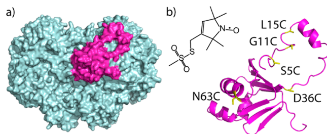
Figure 1. X-ray crystal structure of H ox –2B complex (Protein Data Bank (PDB) ID 4GAM). (a) View of the structure, with MMOH in cyan and MMOB in magenta. There is a second MMOB bound on the other side of MMOH. (b) Structure of the spin label, MTSL. Also depicted is MMOB in the H ox –2B complex, indicating two positions (N63C and D36C) within the core and three (S5C, G11C, and L15C) on the N-terminal tail, labeled for MMOB core-to-tail distance determinations.
