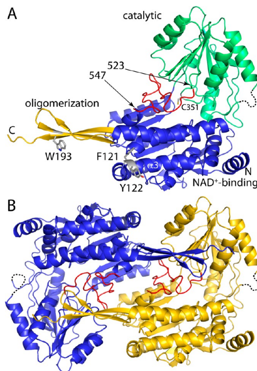
Figure 2. Structure of Put2p. (A) Protomer with the catalytic domain colored green, the NAD + -binding domain blue, and the oligomerization domain gold. The red sections represent the aldehyde-binding loop (transplanted from a MmP5CDH structure), which is disordered in Put2p. Selected side chains of the hexamerization hot spot are colored gray (Trp193, Phe121, and Tyr122). (B) Structure of the Put2p dimer in the asymmetric unit. The two protomers are colored blue and gold. Red sections represent the aldehyde-binding loop, which is disordered in Put2p.
