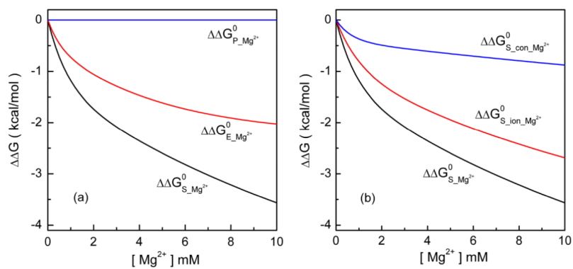
Figure 4. (a) The Mg^{2+} -induced free energy changes: (a) The entropic free energy \Delta\Delta G_S , the Coulomb free energy \Delta\Delta G_E and the polarization energy \Delta\Delta G_P ; (b) The conformational entropy contribution \Delta\Delta G_{S_{conf}} and the ionic entropy contribution \Delta\Delta G_{S_{ion}} .
