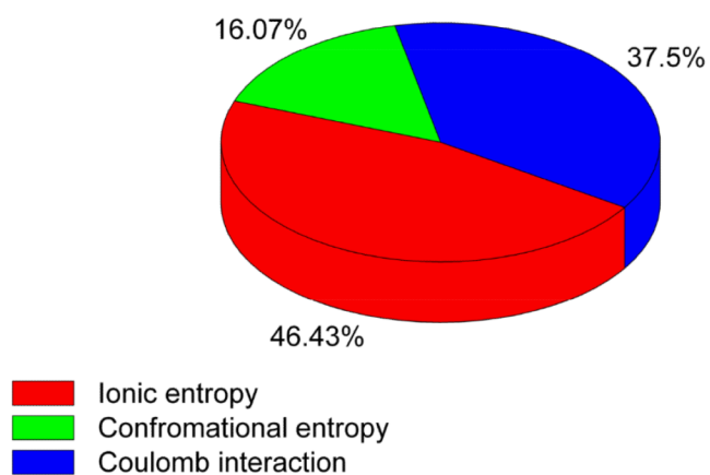
Figure 6. The percentage of each component contribution in the total docking free energy at 10mM [\text{Mg}^{2+}] with 0.1M [\text{Na}^+] background at 37°C.
