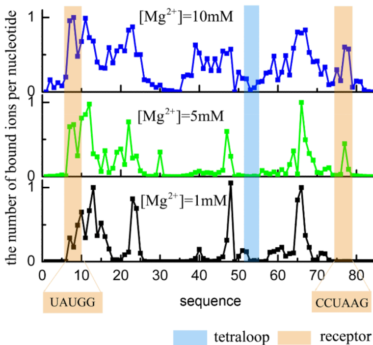
Figure 8. The ion distribution for the lowest energy tetraloop-receptor structure (see Figs. 10b, c and d) in the different Mg^{2+} concentrations with 0.1M NaCl background at 37°C. The distribution is calculated as the Boltzmann average over all the possible ion binding models for the given RNA structure.
