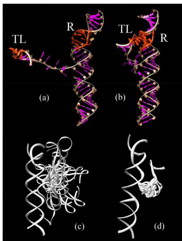
Figure 2. Representative structures for (a) the undocked state and (b) the docked state. “TL” represents the GAAA tetraloop, and “R” represents the receptor, both the GAAA tetraloop and the receptor parts are marked with red color. (c) and (d) show the conformational ensemble of the undocked and the docked states, respectively.
