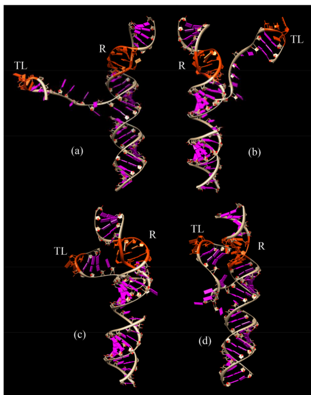
Figure 10. The undocked structures with the lowest electrostatic free energy in the different \text{Mg}^{2+} concentrations with the fixed background of 0.1M NaCl: (a) 0mM, (b) 1mM, (c) 5mM and (d) 10mM.
