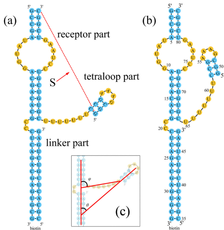
Figure 1. The GAAA tetraloop-receptor system. The GAAA tetraloop and the receptor are connected by a U7 single-stranded linker. (a) The undocked state; (b) The docked state; (c) The definition of the structure parameters \theta and \phi .
