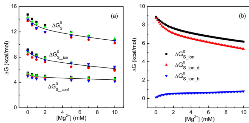
Figure 5. The different components of the entropic free energy. (a) \Delta G_{S_{ion}}^0 and \Delta G_{S_{conf}}^0 are the free energies for the ion entropy and the conformational entropy, respectively. (b) The different components for the ion entropic free energies \Delta G_{S_{ion}}^0 : the diffusive ions \Delta G_{S_{ion_d}}^0 and the bound ions \Delta G_{S_{ion_b}}^0 .
