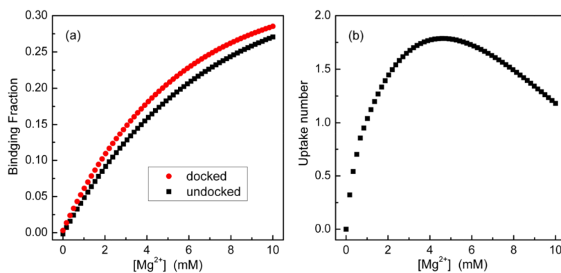
Figure 7. (a) The binding fraction for the docked and the undocked states as a function of the Mg^{2+} concentration in the background of 0.1M NaCl at 37°C. (b) The uptake number of Mg^{2+} as a function of [Mg^{2+}] .
