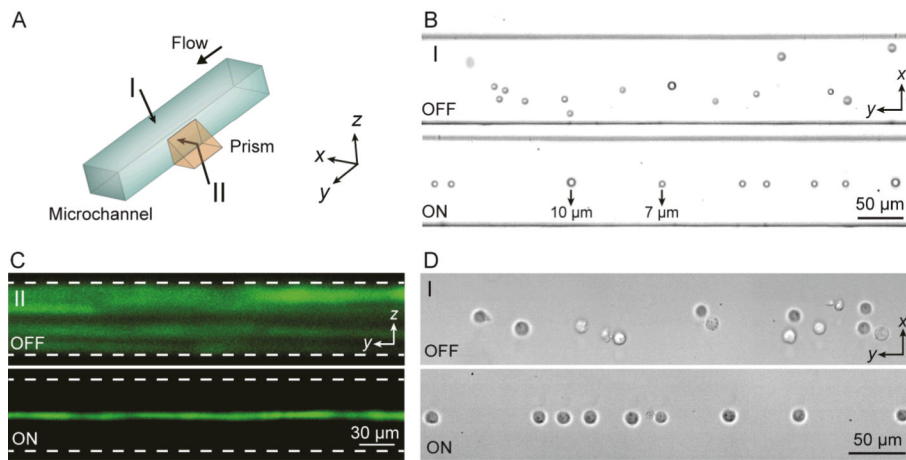
Fig. 2. (A) SSW-based 3D particle focusing observed from different perspectives (I: top view, II: side view). (B) Top-view bright field images and (C) side-view fluorescent stacking images of the particle flow pattern without (OFF) and with (ON) SSW focusing. The dashed lines in (C) indicate the channel boundaries. (D) Top-view images showing cell focusing by SSW. Please refer to Supplementary Video 1.
