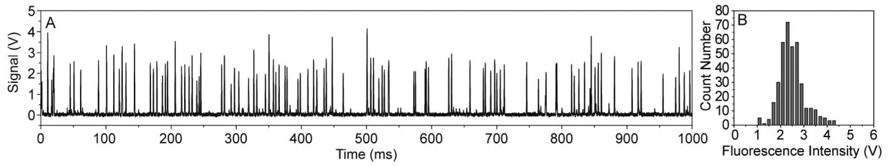
Fig. 6. (A) A data plot of fluorescent peak signals showing the measurement of HL-60 cell with the SSAW-based microfluidic cytometer. (B) The distribution of peak intensities recorded over 4 s using SSAW focusing.
