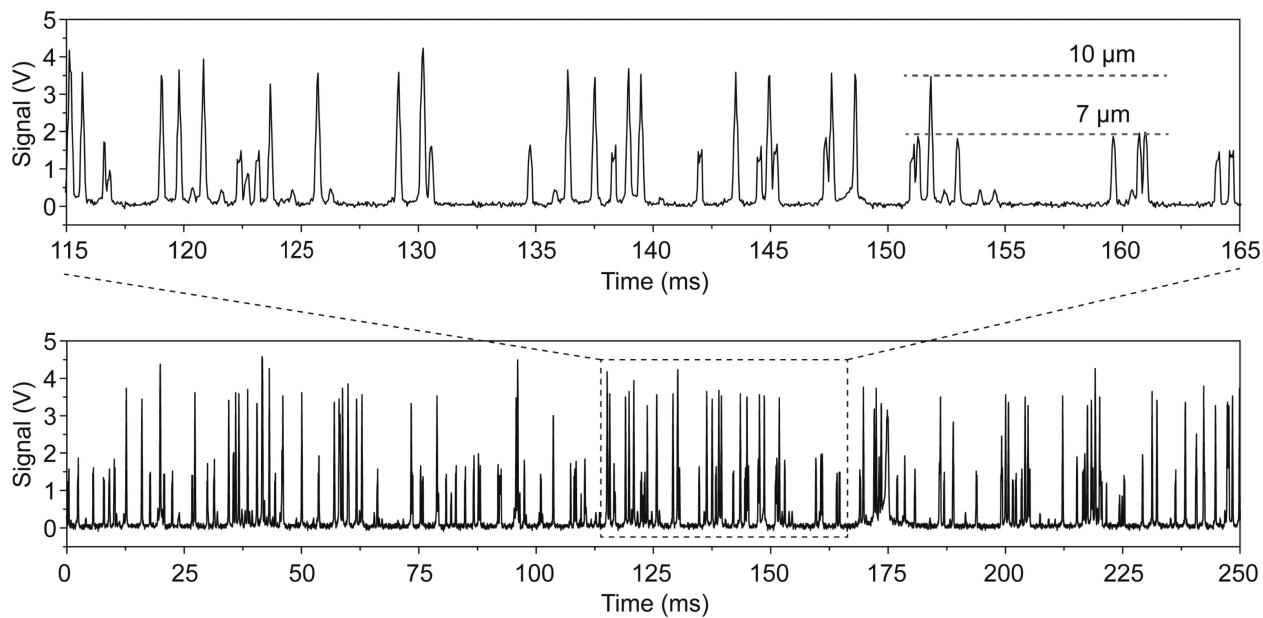
Fig. 4. A data plot of fluorescent peak signals (bottom plot) showing the simultaneous measurement of two types of microparticles with different diameters (7 and 10 \mu\text{m} ). The upper inset is an exploded plot focusing on a time interval of only 50 ms where the signal levels from different diameter particles is clearly visible.
