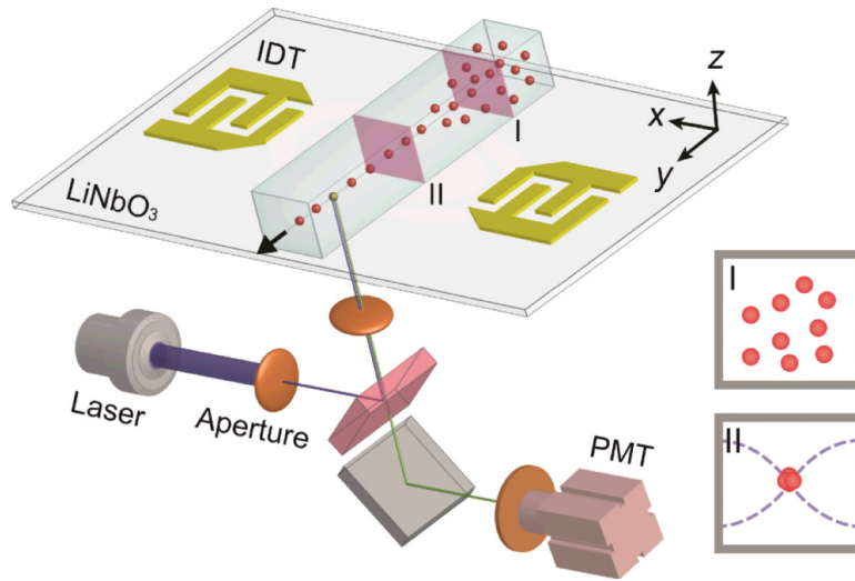
Fig. 1. Schematic of the SSAW-based microfluidic cytometer. A microfluidic device is integrated with a LIF detection system. The insets illustrate cross-sectional views of particle flow patterns before (I) and after (II) SSAW focusing.
