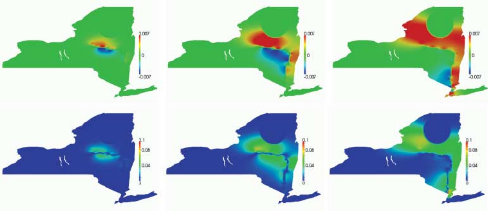
Figure 5. Effect on the propagation front of including landscape heterogeneities at (left to right) 12, 24, and 36 months. Top row: I_{noRiver} - I_{base} . Bottom row: relative difference (I_{noRiver} - I_{base})/I_{noRiver} .
