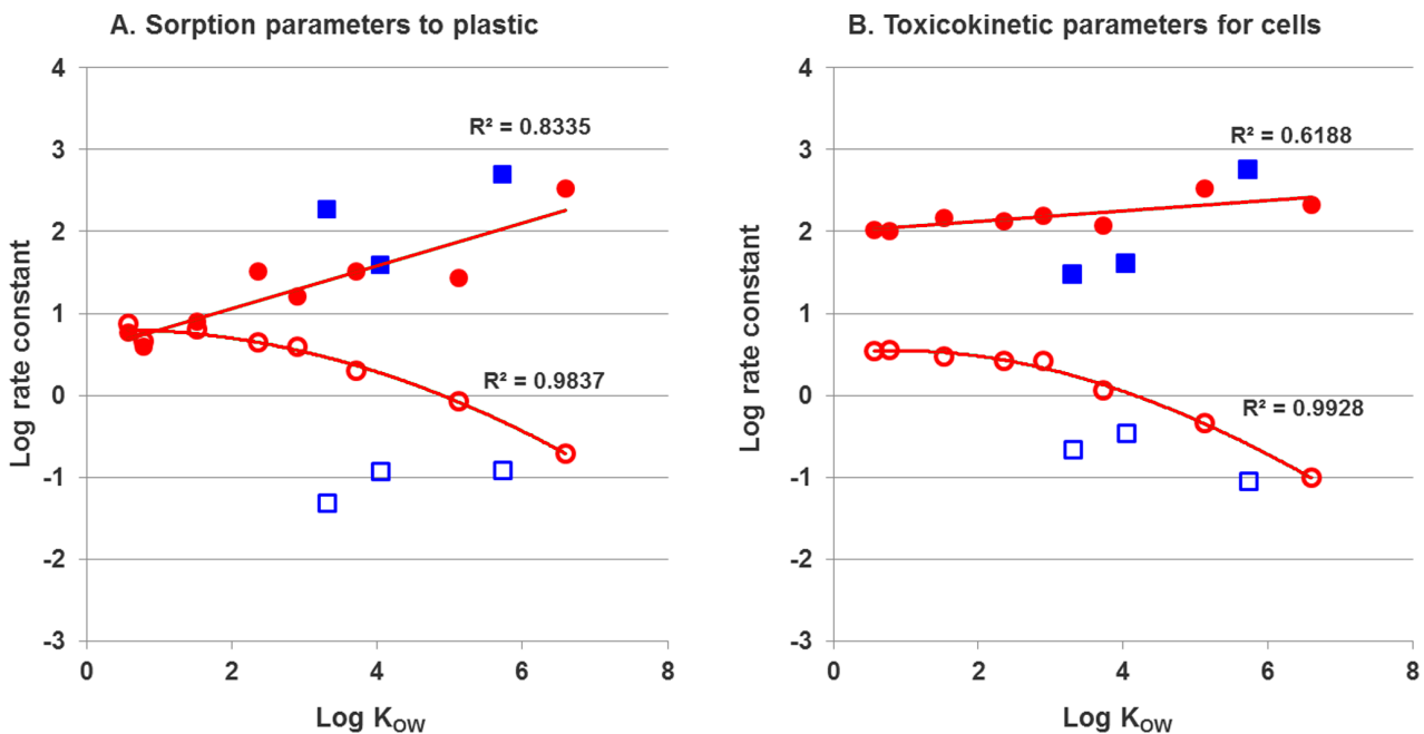
Figure 3. Regression of model parameters and log K_{OW} for non-volatile (red \circ – log k_{in} , red \square – log k_{out} ) and volatile (blue \blacksquare – log k_{in} , blue \square – log k_{out} ) compounds. Data for volatile compounds were not used for fitting the model and trend lines. Red — – trend lines for log k_{in} and log k_{out} (A – plastic: log k_{in} = 0.2602 \cdot \log K_{OW} + 0.5385 ; log k_{out} = -0.0388 \cdot (\log K_{OW})^2 + 0.0272 \cdot \log K_{OW} + 0.7982 , B – cells: log k_{in} = 0.0641 \cdot \log K_{OW} + 1.9898 , log k_{out} = -0.0447 \cdot (\log K_{OW})^2 + 0.0619 \cdot \log K_{OW} + 0.525 ). doi:10.1371/journal.pone.0092303.g003
