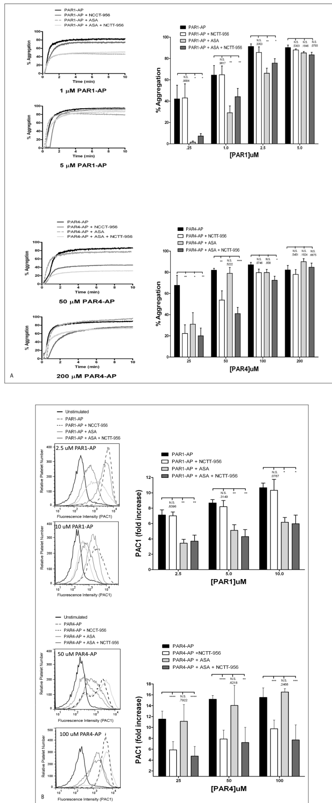
Figure 6. COX-1 and 12-LOX regulation of PAR-mediated platelet activation
