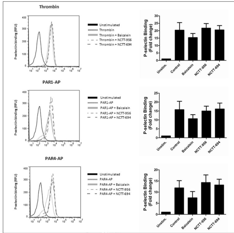
Figure 3. 12-LOX is not critical for agonist-mediated \alpha -granule secretion \alpha -granule secretion was determined following stimulation of platelets with 10 nM thrombin, 20 \mu M PAR1-AP, or 200 \mu M PAR4-AP in the presence or absence of active and inactive 12-LOX inhibitors (N=4). P-selectin expression following treatment with 25 \mu M NCTT-956, 50 \mu M baicalein, or 25 \mu M NCTT-694 was not significantly different from control.
