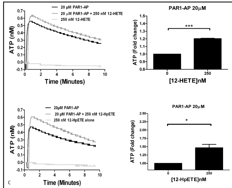
Figure 2. 12-LOX activation is required for dense granule secretion in platelets
