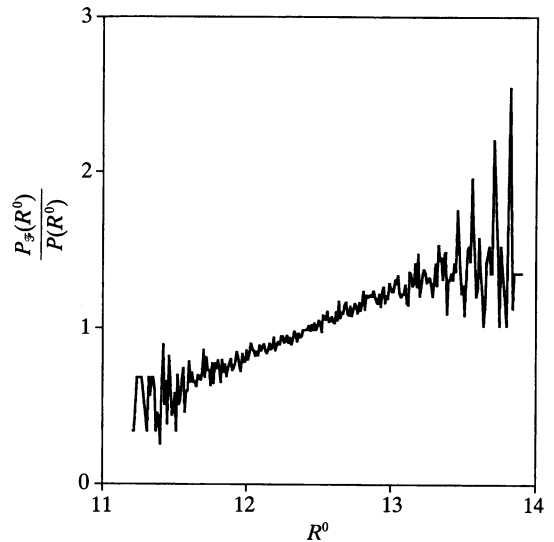
FIG. 3. Probability of the native state structure having a given R^\circ value [ P_{\#}(R^\circ) ] compared with what would be expected at random [ P(R^\circ) ], obtained by choosing 150,000 random sets of interaction parameters for the lattice model as described (20). As expected, structures that are more optimizable with larger values of R^\circ are overrepresented in the set of native structures.
