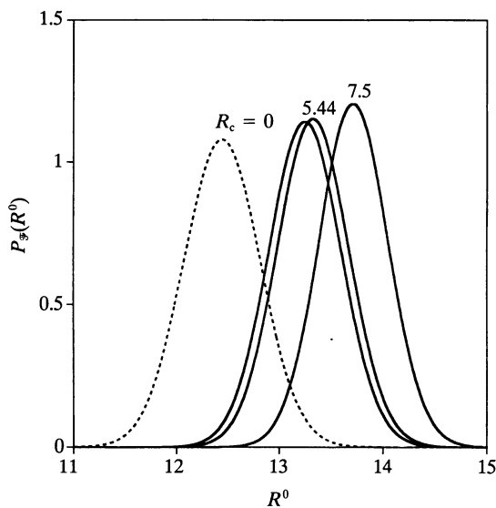
FIG. 2. Distribution of R^\circ values for the native state structures [ P_{\#}(R^\circ) ] expected for various values of R_c (solid lines), compared with the distribution of R^\circ values for all possible structures [ P(R^\circ) ] (dashed line). Even with no evolutionary pressure ( R_c = 0 ), it is still the most optimizable structures that are most likely to result with a random set of interaction parameters. As the evolutionary pressure increases (increasing R_c ), the distribution of the native states moves toward the extreme tail of the P(R^\circ) distribution, resulting in fewer different structures observed.
