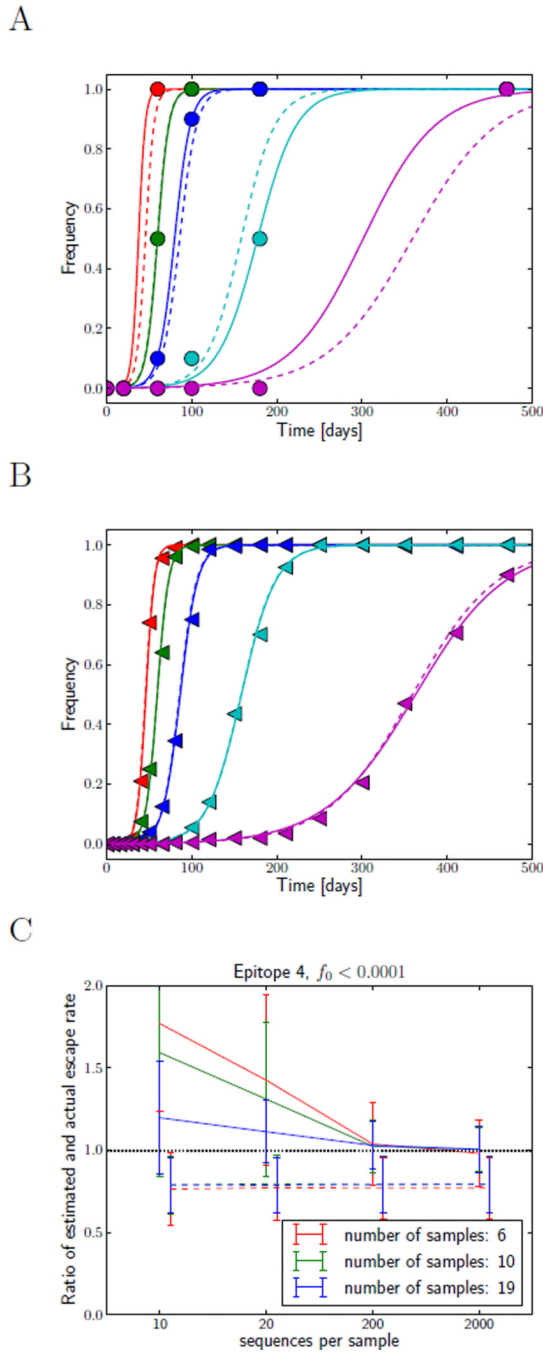
Figure 4. Influence of sampling frequency and sampling depth on fidelity of estimates of the escape rate. Panels A and B show mutation frequencies in population samples for infrequent shallow sampling ( n = 10 , A), and more frequent deep sampling ( n = 200 , B). The actual mutation frequencies are shown as dashed lines, the sample frequencies are indicated by symbols, while the fitted trajectories as solid lines. Obviously, more frequent and deeper sampling will improve the estimates of the escape rate. This is quantified in panel C. It shows the mean estimate of the escape rate of epitope 4 (left pointed triangles) and its standard deviation as a function of sampling depth for different sampling frequencies. The
