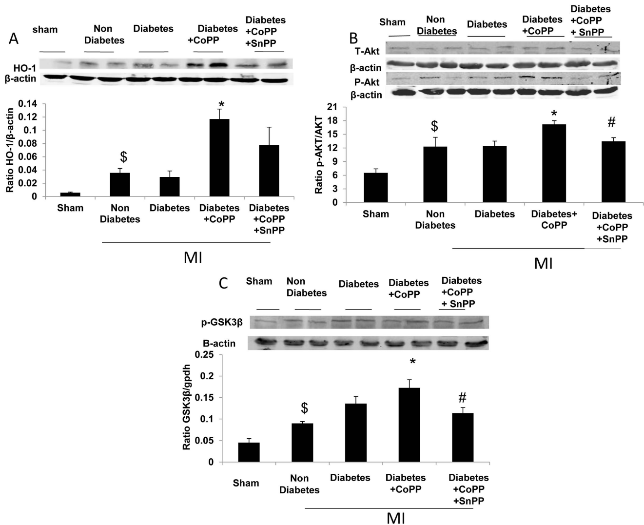
Figure 6. HO-1 induction increases HO-1, AKT and GSK3 \beta expression in diabetic hearts. A: CoPP treatment significantly increased HO-1 expression levels (Means \pm SD, n = 5. ^{\$} p < 0.005 vs. sham, ^* p < 0.01 vs. diabetes.). B: Western blot analysis of AKT and p-AKT and p-Akt/Akt ratio in the different groups. CoPP treatment increased p-Akt levels while SnPP decreased the expression of p-AKT compared to the CoPP treated diabetic mice. (Means \pm SD, n = 5. ^{\$} < 0.05 vs. sham, ^* p < 0.05 vs. diabetes, ^{\#} p < 0.05 vs. diabetes+CoPP) C: Western blot analysis of GSK-3 \beta in mice subjected to LAD ligation. CoPP treatment led to an increase in GSK-3 \beta levels; SnPP decreased GSK-3 \beta expression compared to the CoPP treated diabetic mice (Means \pm SD, n = 5. ^{\$} < 0.05 vs. sham, ^* p < 0.05 vs. diabetes, ^{\#} p < 0.05 vs. diabetes+CoPP). doi:10.1371/journal.pone.0092246.g006
