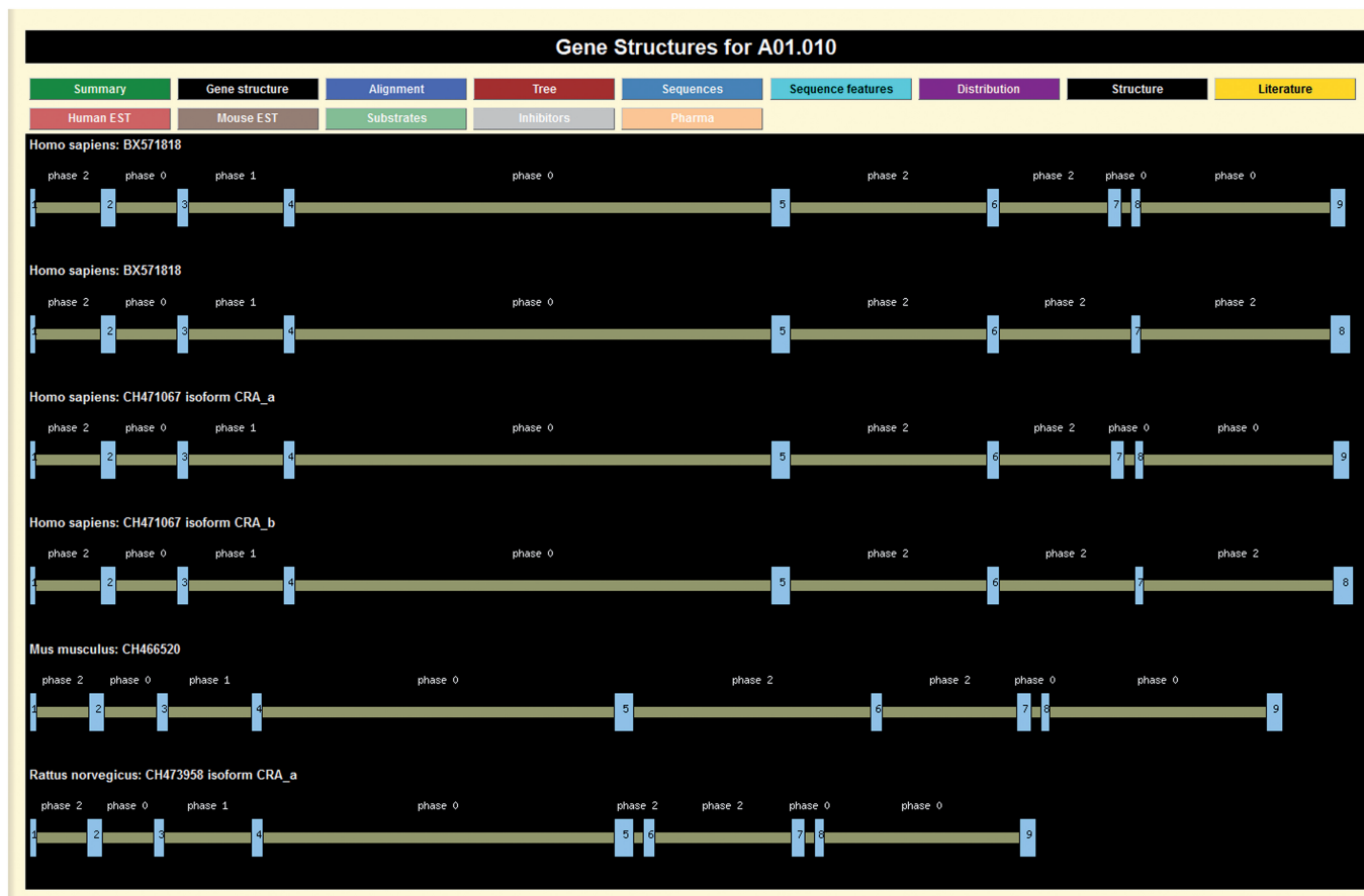
Figure 3. Example of a gene structure. The gene structures for cathepsin E (MEROPS identifier A01.010) are shown.
