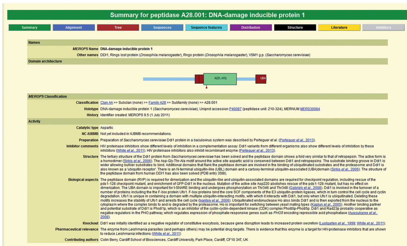
Figure 2. Example of a complete peptidase summary. The summary for DNA-damage inducible protein 1 (MEROPS identifier A28.001) is shown. The summary was kindly supplied by Dr Colin Berry.
