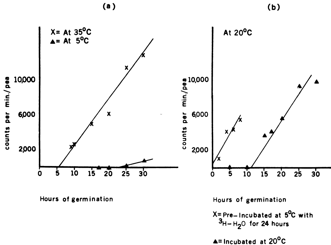
FIG. 1. Incorporation of 3 H-H 2 O into fatty acids of germinating pea.
