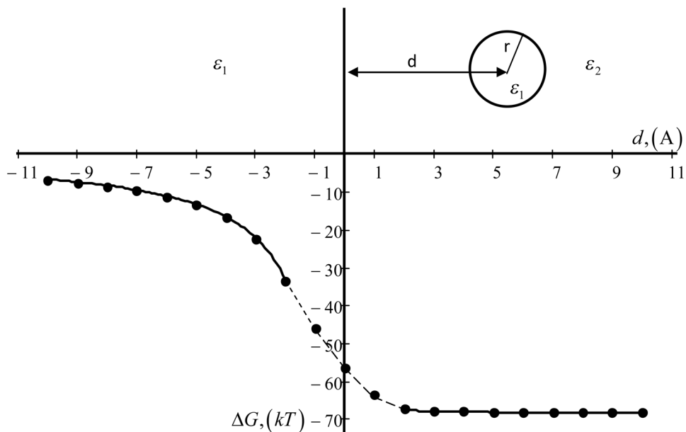
Figure 5. Total energy of a spherical shell of charge as a function of its position relative to a planar dielectric boundary. \epsilon_2 = 80 , \epsilon_1 = 2 , r = 2\text{\AA} . Solid line is an analytical result (7) and (8), points are result from Delphi. Of course equations (7) and (8) are not valid for overlapping area in the region -r < d < r .
