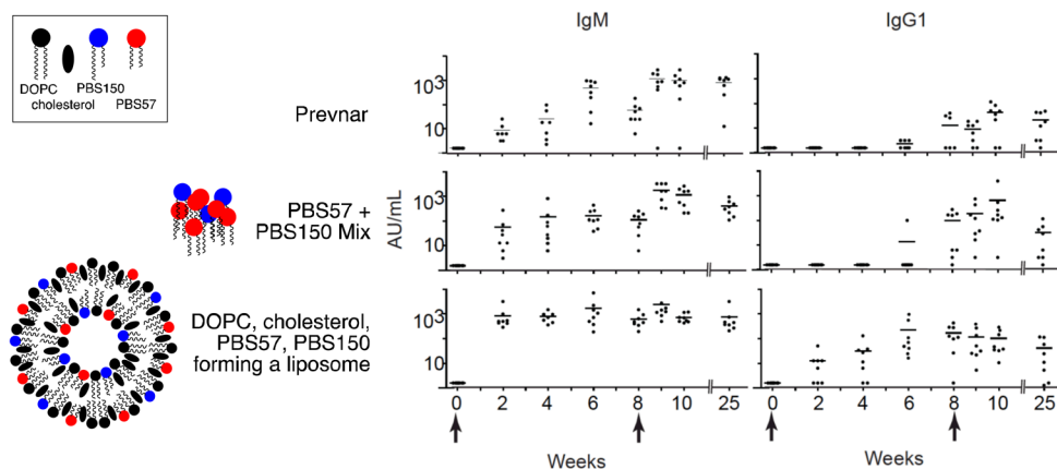
Figure 3. Antibody (IgM and IgG1) formation in response to vaccination (intraperitoneal injection on days 0 and 57) with Pevnar13 20 (2.2 \mu g of each polysaccharide) or with PBS57+PBS150 as a simple mixture (4 \mu g of PBS150 and 1 \mu g of PBS57) or in liposome formulation, as indicated. Each injection contained an equivalent amount of pneumococcal polysaccharide serotype 14. Sera were collected at indicated intervals to measure IgM and IgG1 antibody titers against S. pneumoniae serotype 14. Each dot represents the serum titer of an individual mouse at the indicated time. Statistical analysis: * p-value < 0.05; *** p-value < 0.001. The first time periods at which p-values below 0.05 or 0.001 are indicated.
