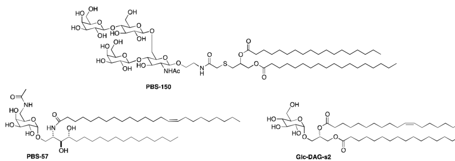
Figure 2. Structures of NKT cell agonists PBS57 and Glc-DAG-s2 and lipitated tetrasaccharide PBS150.
