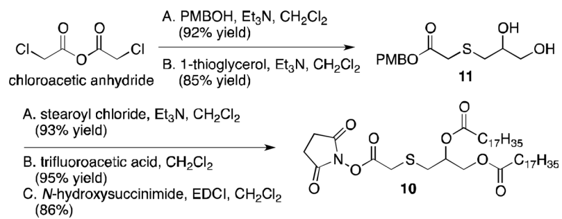
Scheme 2. Synthesis of 10 .
